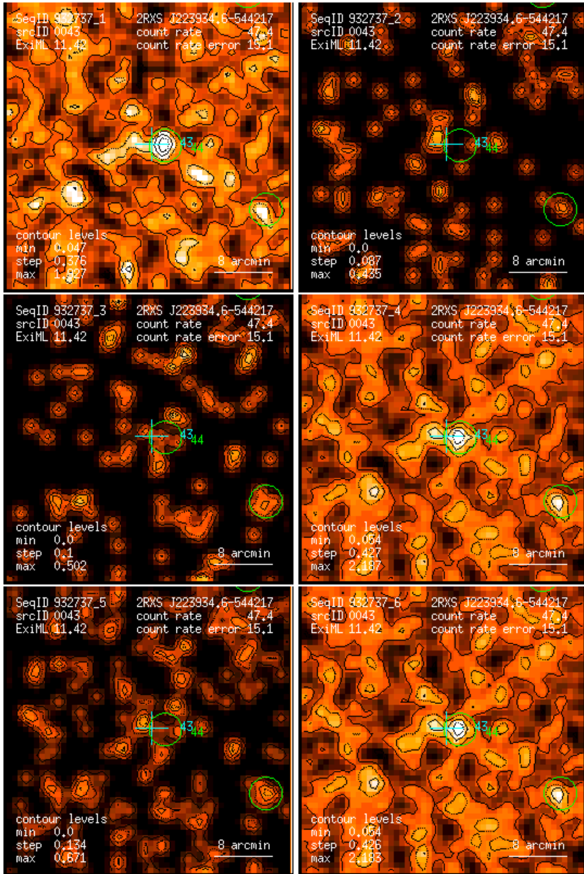
Figure 43: RASS 932737: detection 0043: band rate images, Gaussian filter: (1) PSPC channels 11 – 41, (2) 52 – 90, (3) 91 – 201, (4) 11 – 235, (5) 52 – 201, (6) 11 – 201. Broad band rates in counts/ks. Band rate contour levels in counts/ks/arcmin 2 .
