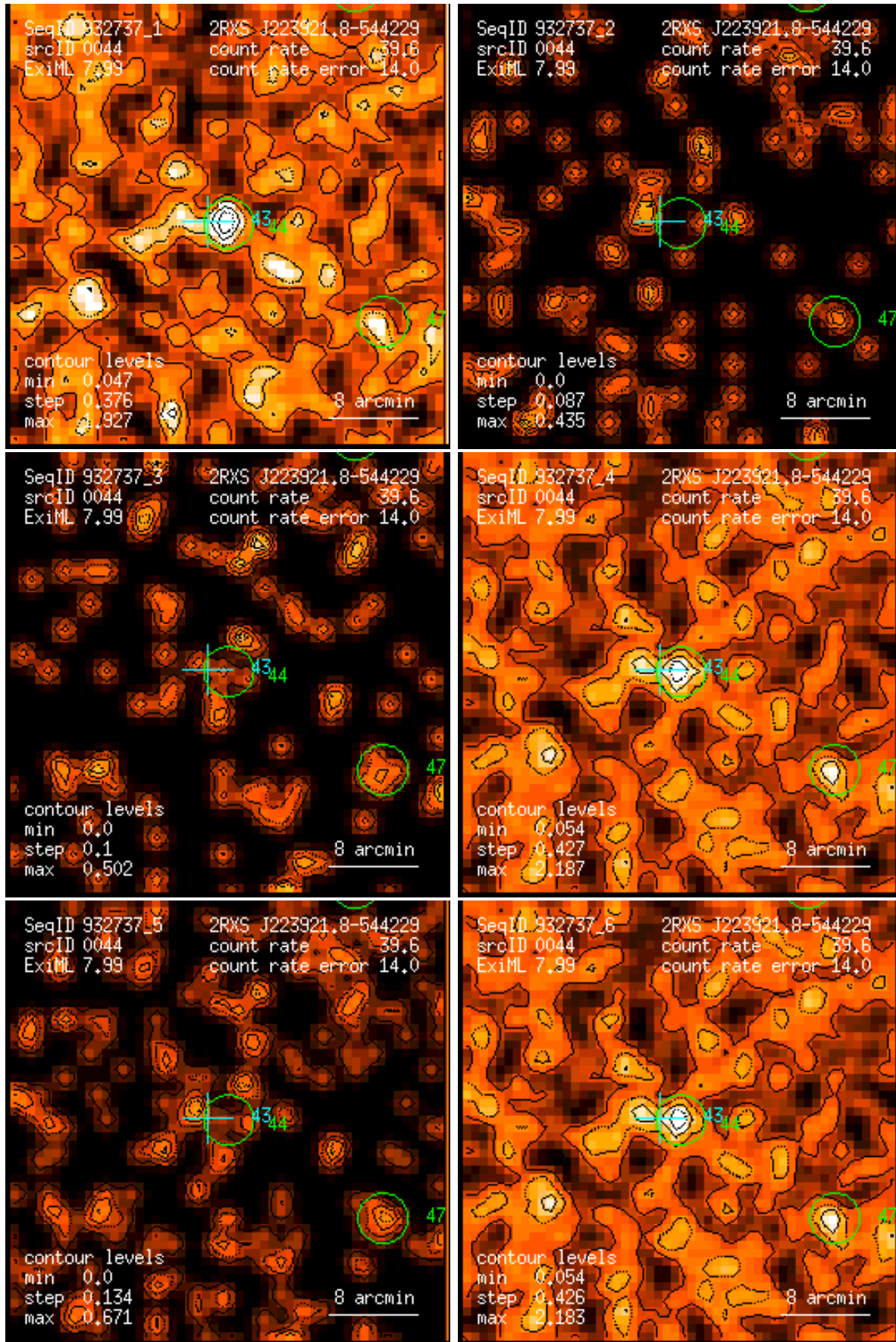
Figure 44: RASS 932737: detection 0044: band rate images, Gaussian filter: (1) PSPC channels 11 – 41, (2) 52 – 90, (3) 91 – 201, (4) 11 – 235, (5) 52 – 201, (6) 11 – 201. Broad band rates in counts/ks. Band rate contour levels in counts/ks/arcmin 2 .
