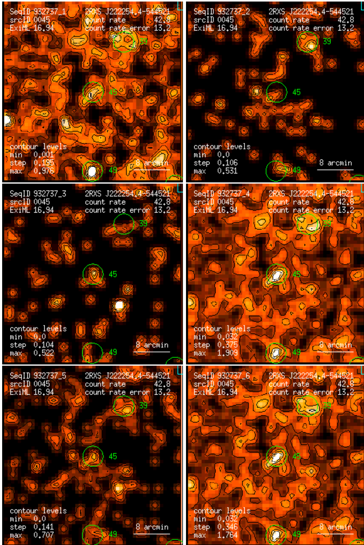
Figure 45: RASS 932737: detection 0045: band rate images, Gaussian filter: (1) PSPC channels 11 – 41, (2) 52 – 90, (3) 91 – 201, (4) 11 – 235, (5) 52 – 201, (6) 11 – 201. Broad band rates in counts/ks. Band rate contour levels in counts/ks/arcmin 2 .
