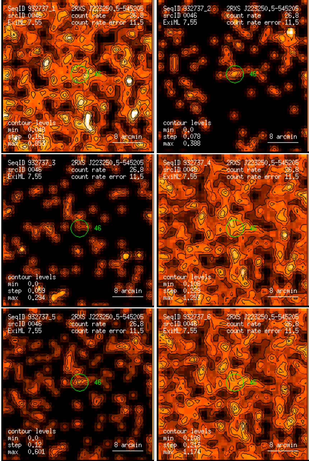
Figure 46: RASS 932737: detection 0046: band rate images, Gaussian filter: (1) PSPC channels 11 – 41, (2) 52 – 90, (3) 91 – 201, (4) 11 – 235, (5) 52 – 201, (6) 11 – 201. Broad band rates in counts/ks. Band rate contour levels in counts/ks/arcmin 2 .
