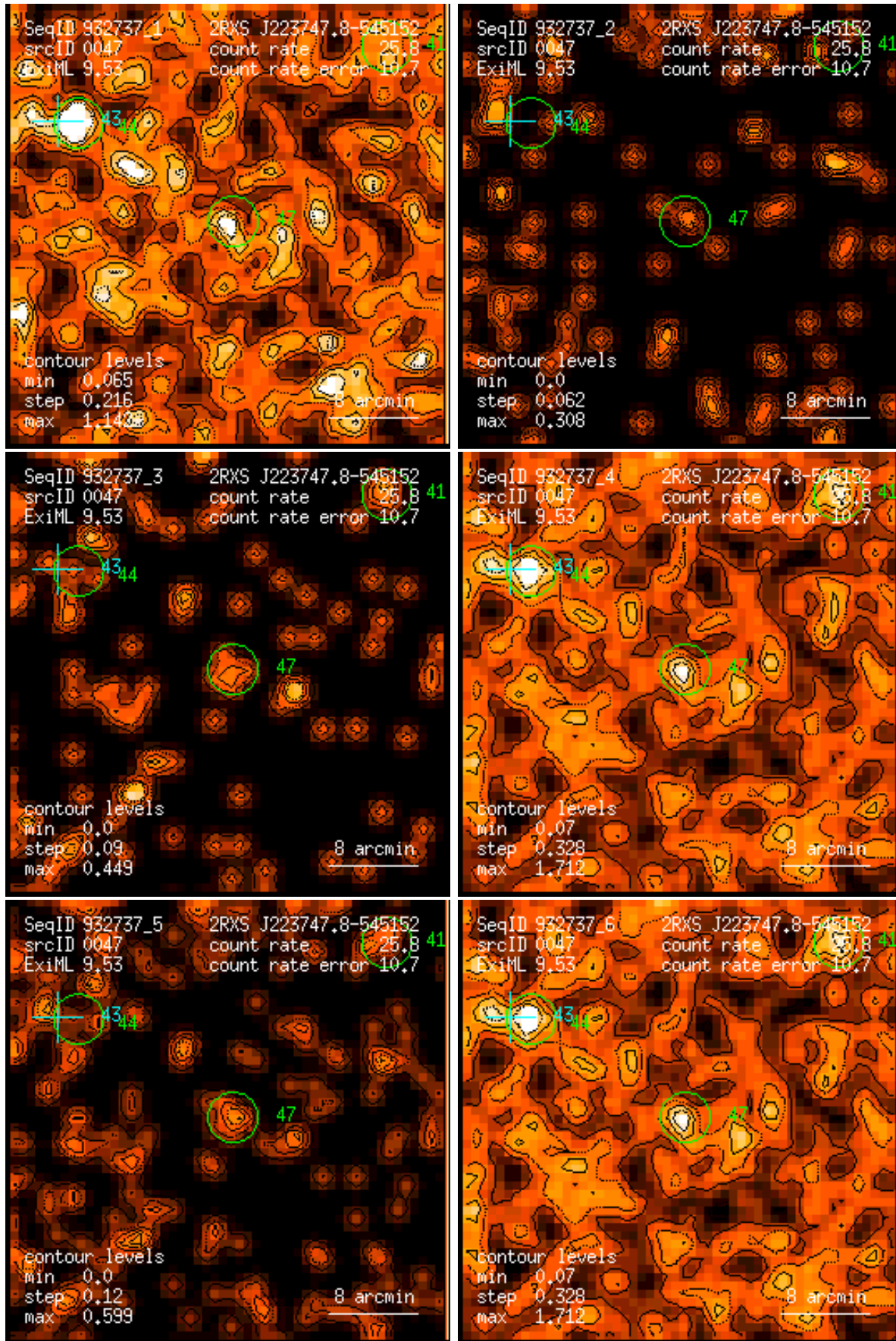
Figure 47: RASS 932737: detection 0047: band rate images, Gaussian filter: (1) PSPC channels 11 – 41, (2) 52 – 90, (3) 91 – 201, (4) 11 – 235, (5) 52 – 201, (6) 11 – 201. Broad band rates in counts/ks. Band rate contour levels in counts/ks/arcmin 2 .
