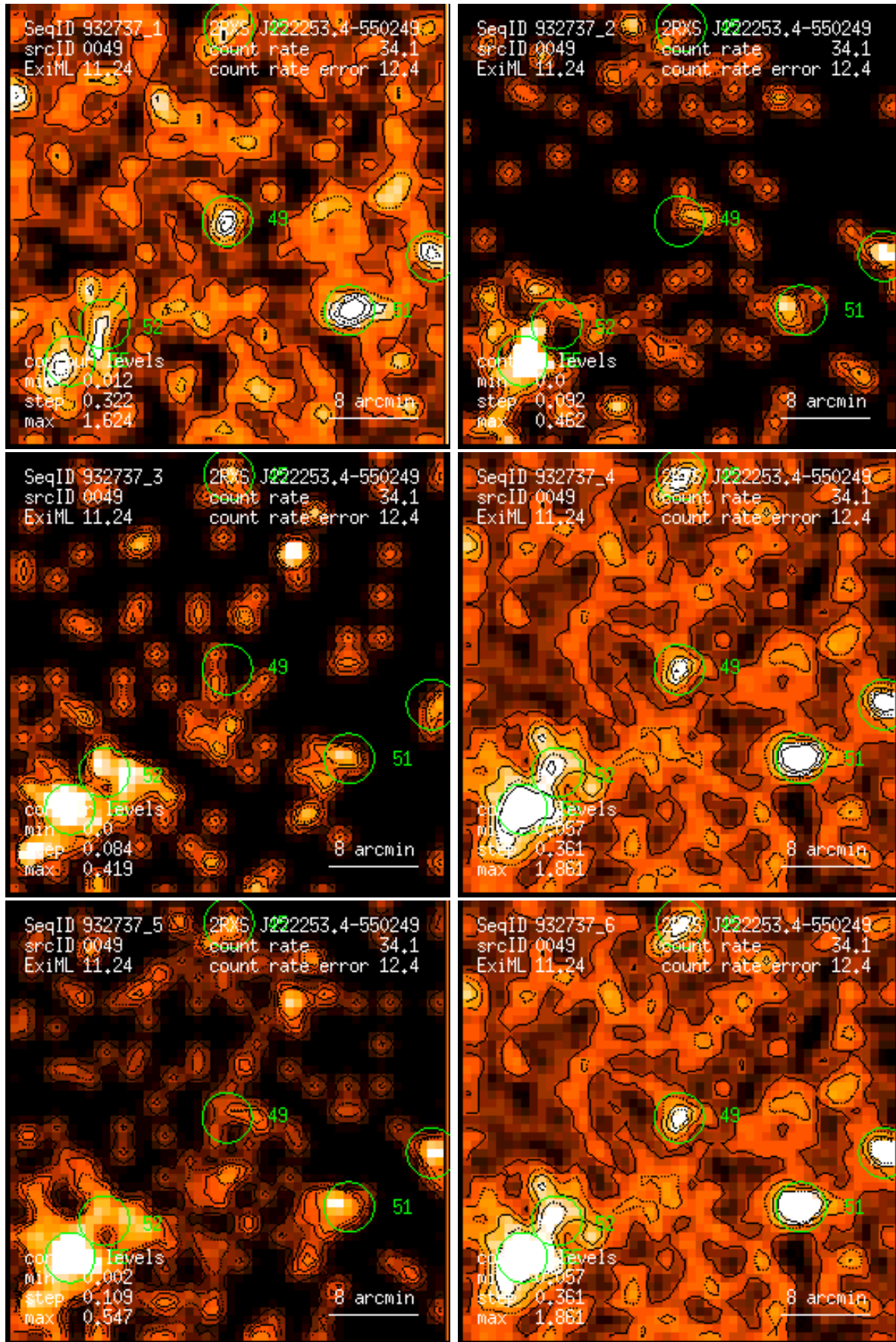
Figure 49: RASS 932737: detection 0049: band rate images, Gaussian filter: (1) PSPC channels 11 – 41, (2) 52 – 90, (3) 91 – 201, (4) 11 – 235, (5) 52 – 201, (6) 11 – 201. Broad band rates in counts/ks. Band rate contour levels in counts/ks/arcmin 2 .
