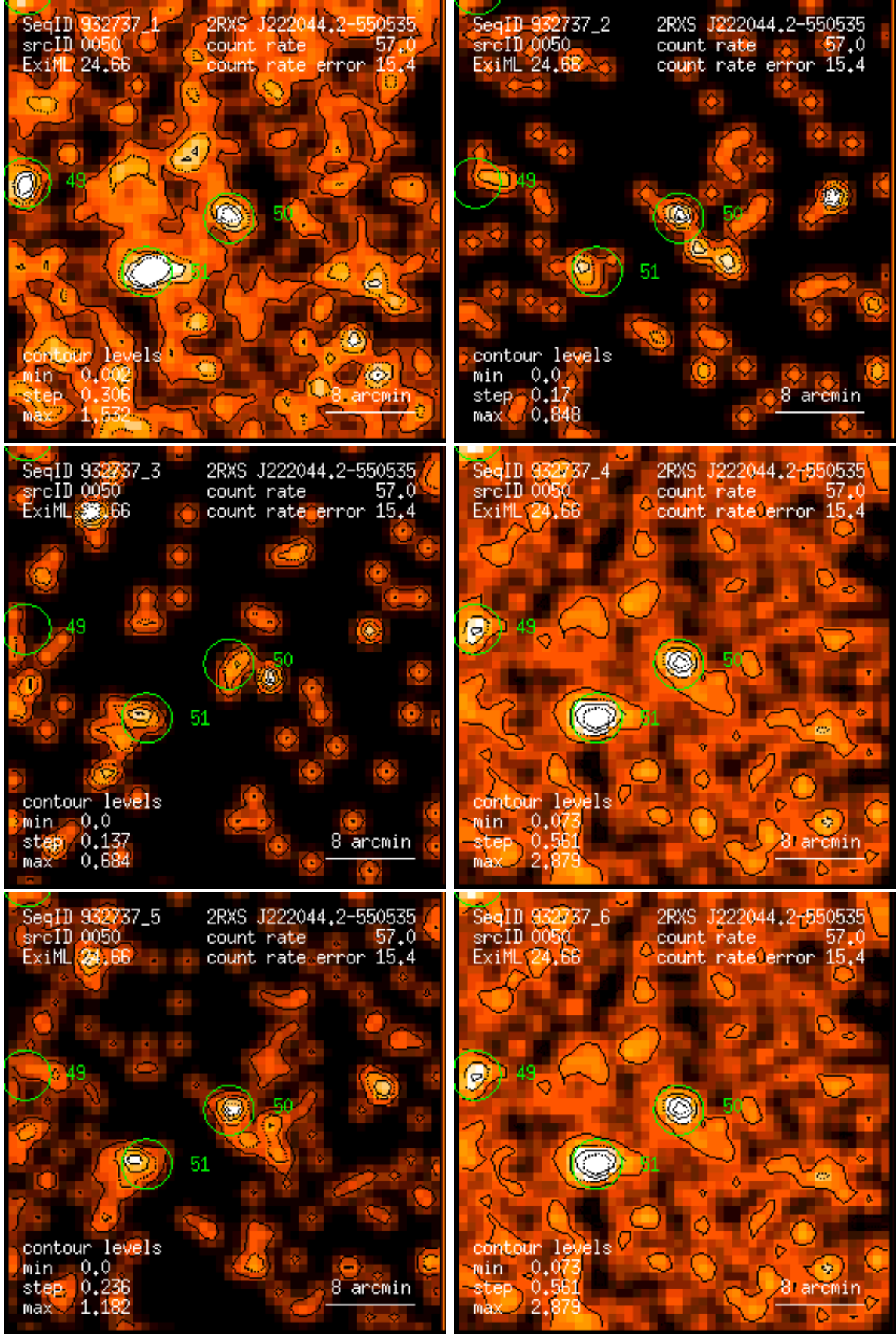
Figure 50: RASS 932737: detection 0050: band rate images, Gaussian filter: (1) PSPC channels 11 – 41, (2) 52 – 90, (3) 91 – 201, (4) 11 – 235, (5) 52 – 201, (6) 11 – 201. Broad band rates in counts/ks. Band rate contour levels in counts/ks/arcmin 2 .
