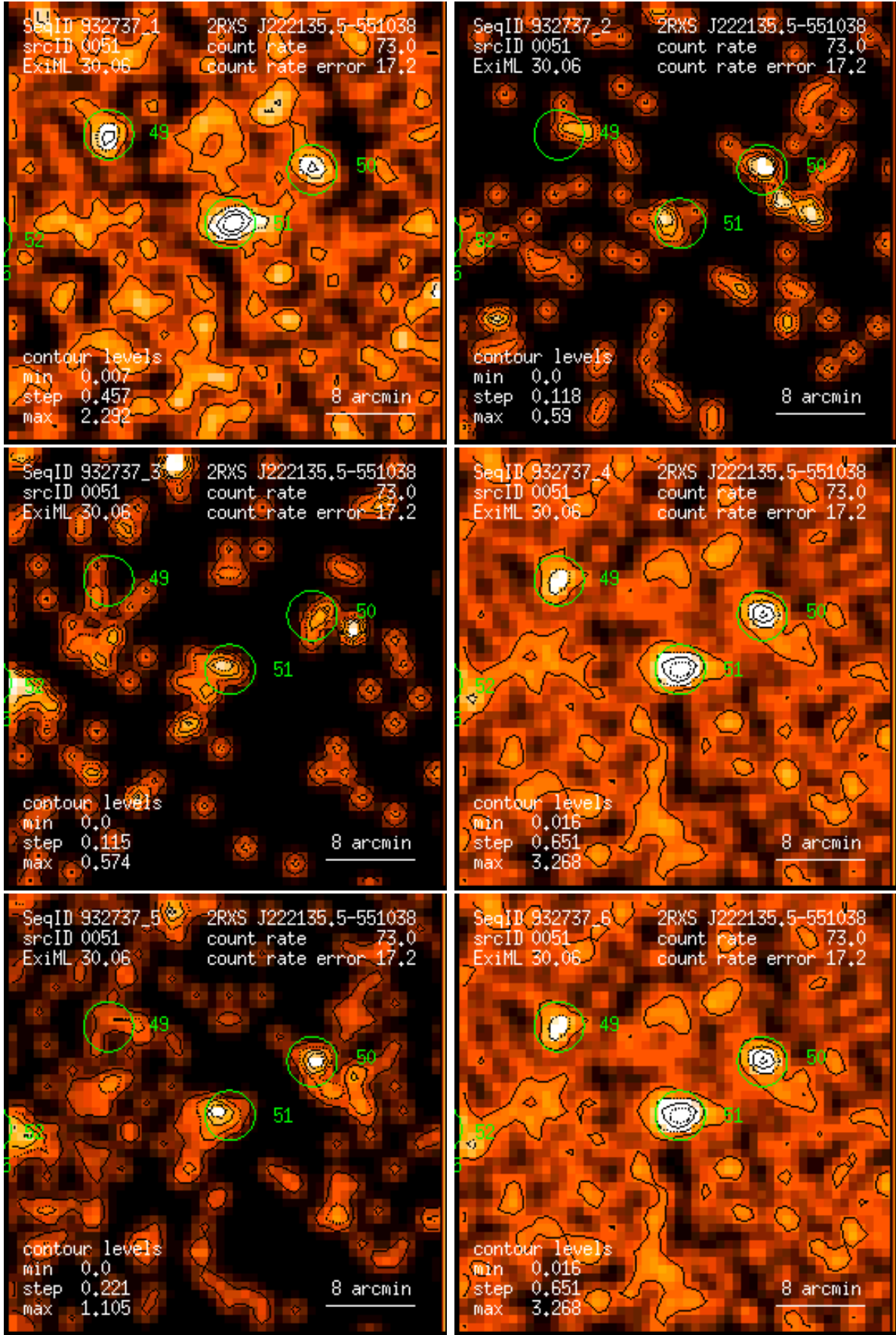
Figure 51: RASS 932737: detection 0051: band rate images, Gaussian filter: (1) PSPC channels 11 – 41, (2) 52 – 90, (3) 91 – 201, (4) 11 – 235, (5) 52 – 201, (6) 11 – 201. Broad band rates in counts/ks. Band rate contour levels in counts/ks/arcmin 2 .
