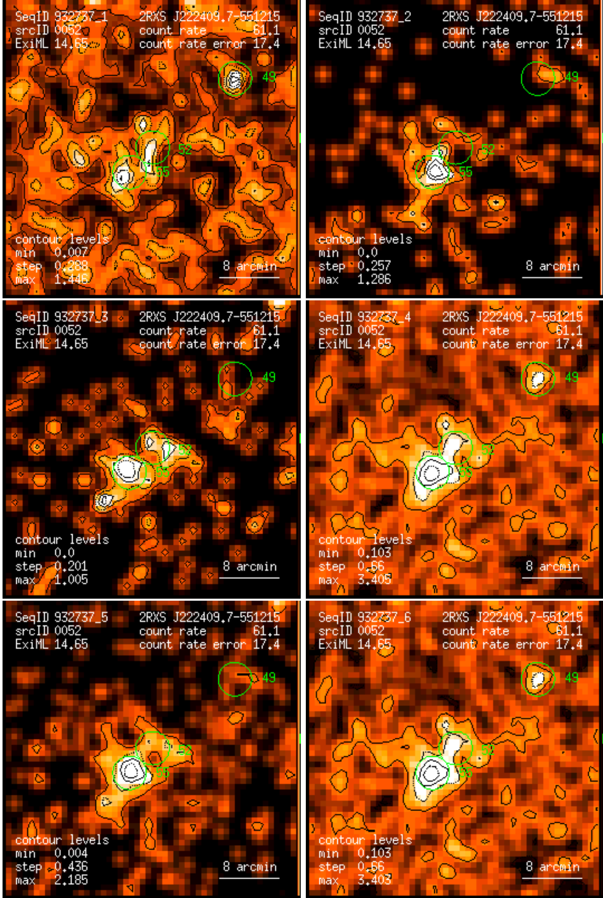
Figure 52: RASS 932737: detection 0052: band rate images, Gaussian filter: (1) PSPC channels 11 – 41, (2) 52 – 90, (3) 91 – 201, (4) 11 – 235, (5) 52 – 201, (6) 11 – 201. Broad band rates in counts/ks. Band rate contour levels in counts/ks/arcmin 2 .
