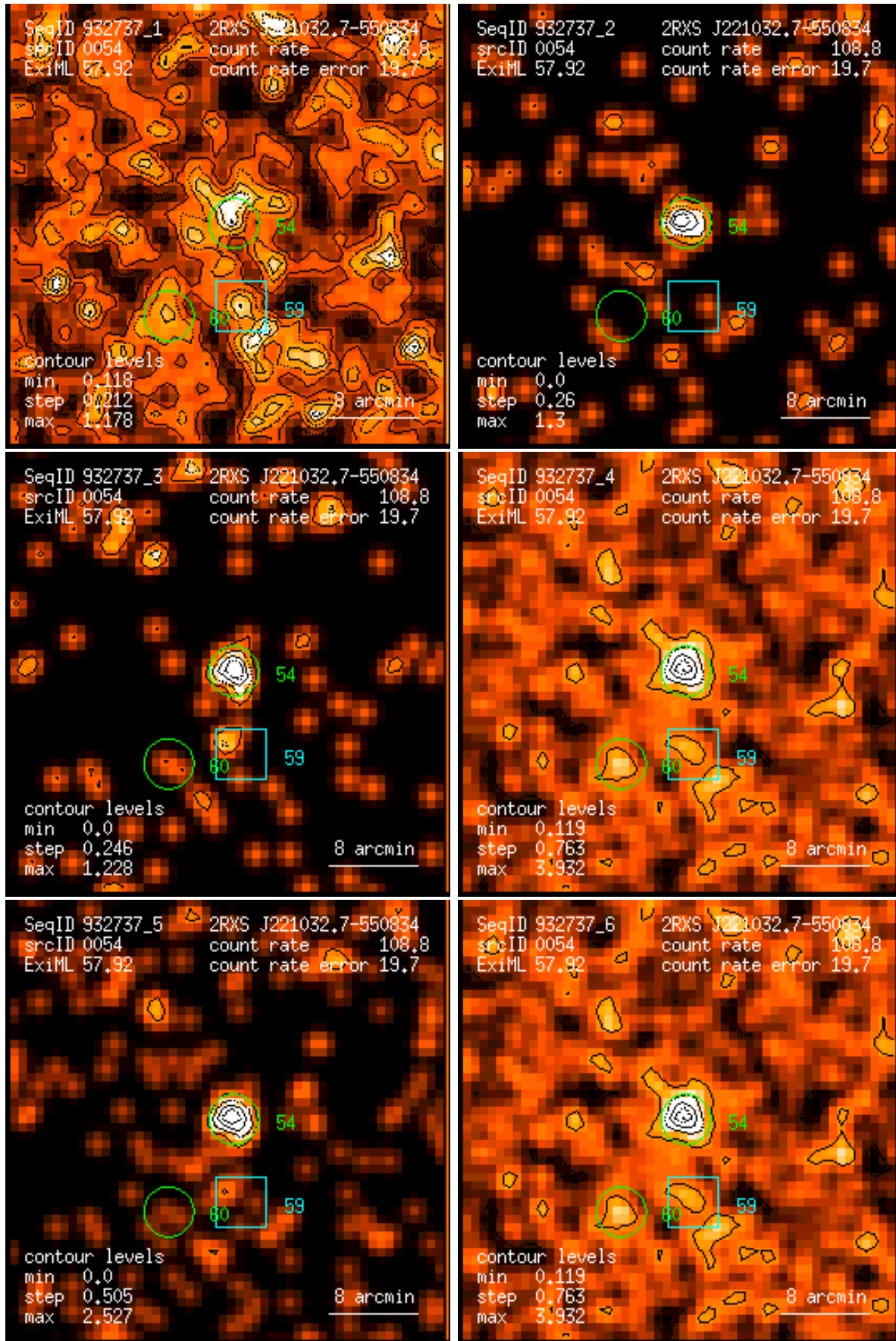
Figure 54: RASS 932737: detection 0054: band rate images, Gaussian filter: (1) PSPC channels 11 – 41, (2) 52 – 90, (3) 91 – 201, (4) 11 – 235, (5) 52 – 201, (6) 11 – 201. Broad band rates in counts/ks. Band rate contour levels in counts/ks/arcmin 2 .
