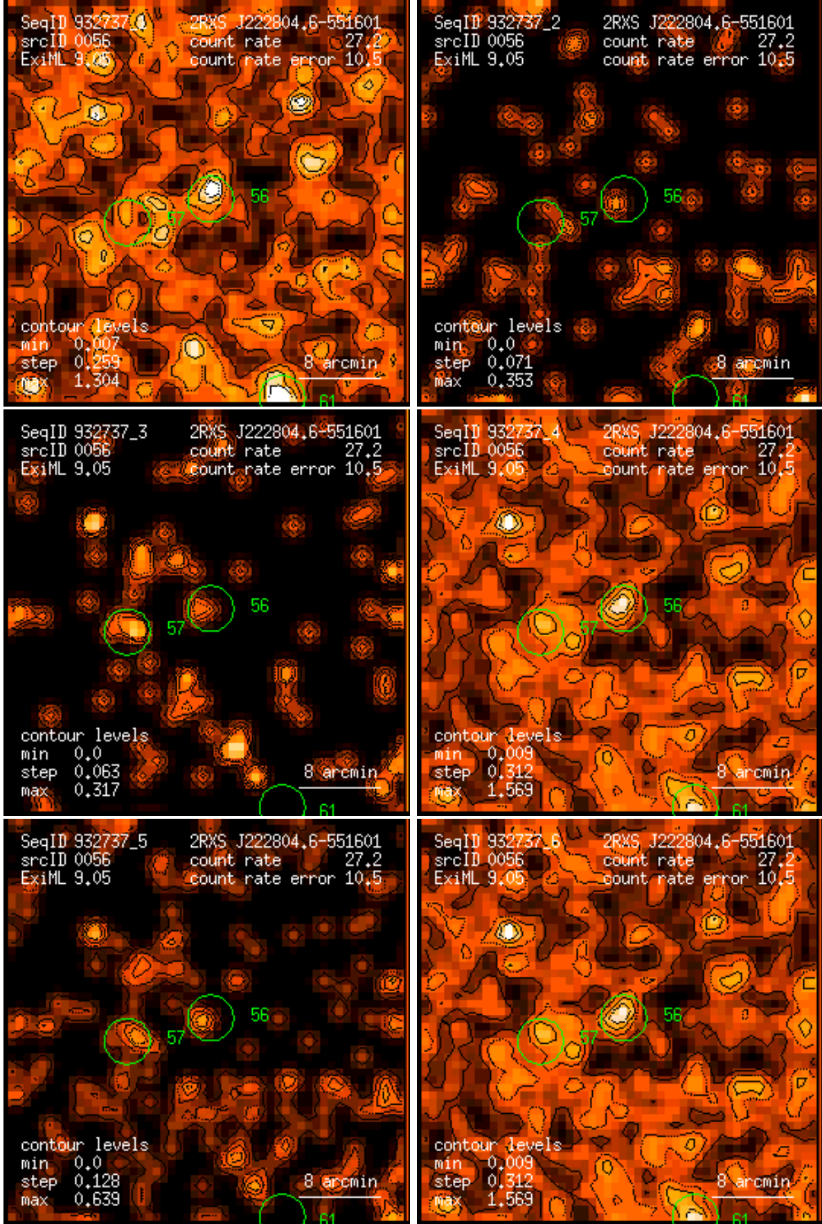
Figure 56: RASS 932737: detection 0056: band rate images, Gaussian filter: (1) PSPC channels 11 – 41, (2) 52 – 90, (3) 91 – 201, (4) 11 – 235, (5) 52 – 201, (6) 11 – 201. Broad band rates in counts/ks. Band rate contour levels in counts/ks/arcmin 2 .
