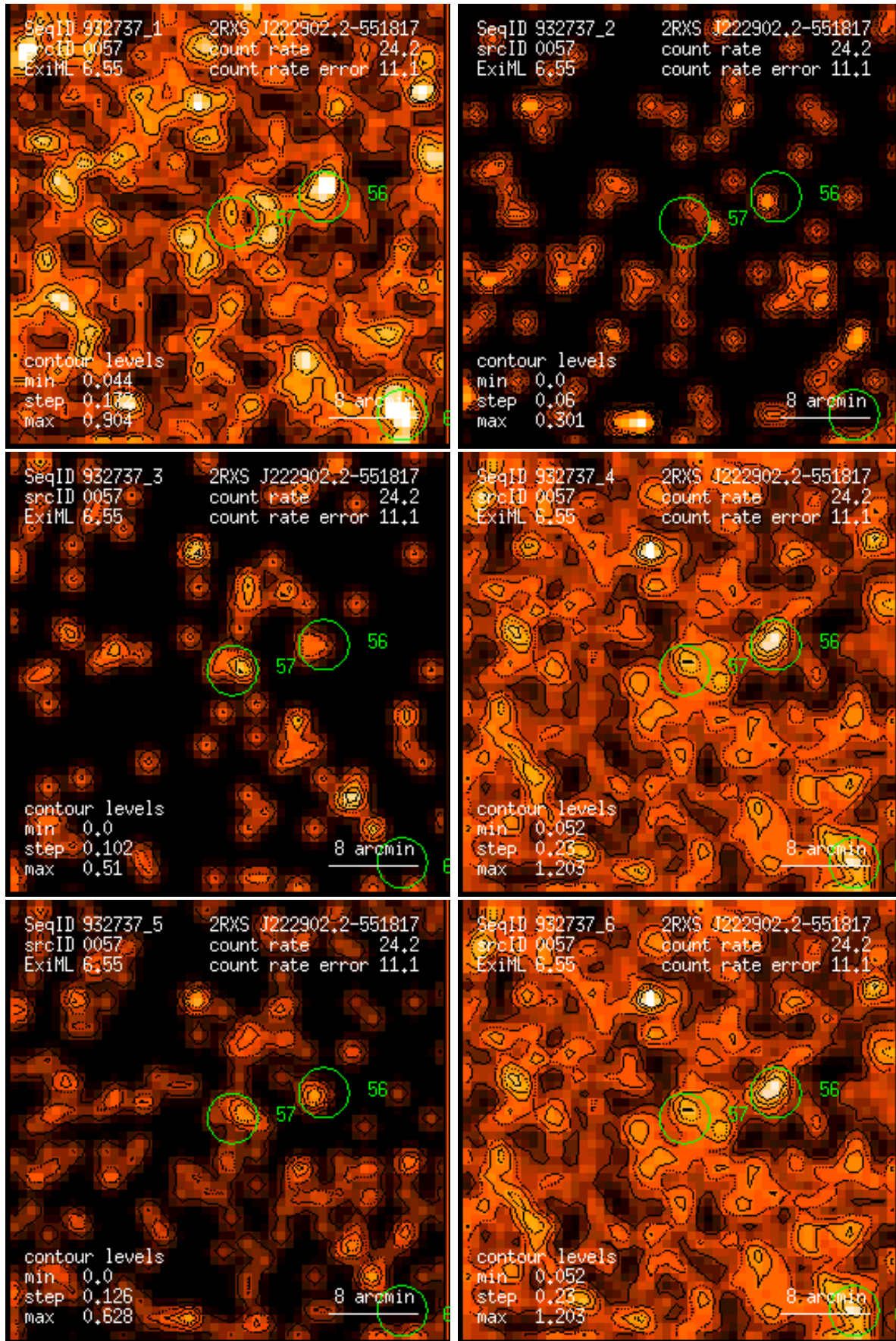
Figure 57: RASS 932737: detection 0057: band rate images, Gaussian filter: (1) PSPC channels 11 – 41, (2) 52 – 90, (3) 91 – 201, (4) 11 – 235, (5) 52 – 201, (6) 11 – 201. Broad band rates in counts/ks. Band rate contour levels in counts/ks/arcmin 2 .
