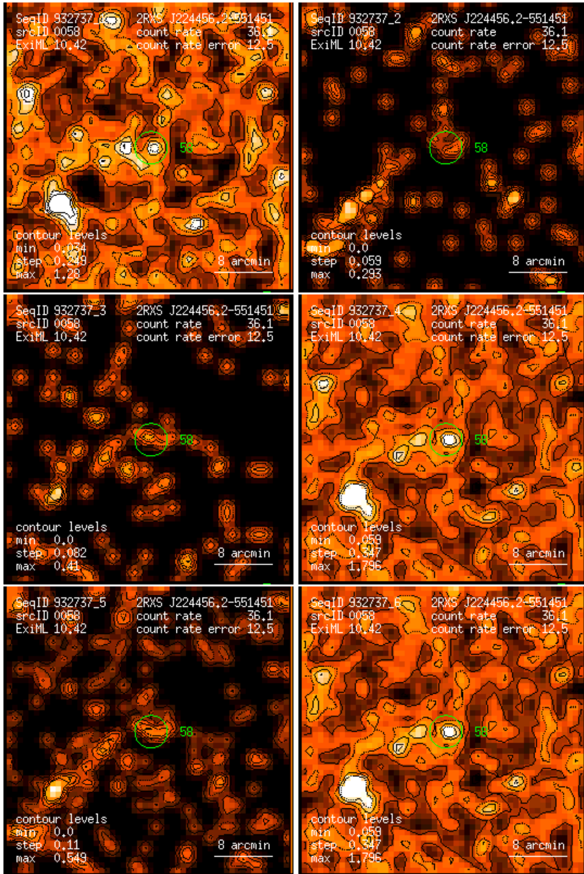
Figure 58: RASS 932737: detection 0058: band rate images, Gaussian filter: (1) PSPC channels 11 – 41, (2) 52 – 90, (3) 91 – 201, (4) 11 – 235, (5) 52 – 201, (6) 11 – 201. Broad band rates in counts/ks. Band rate contour levels in counts/ks/arcmin 2 .
