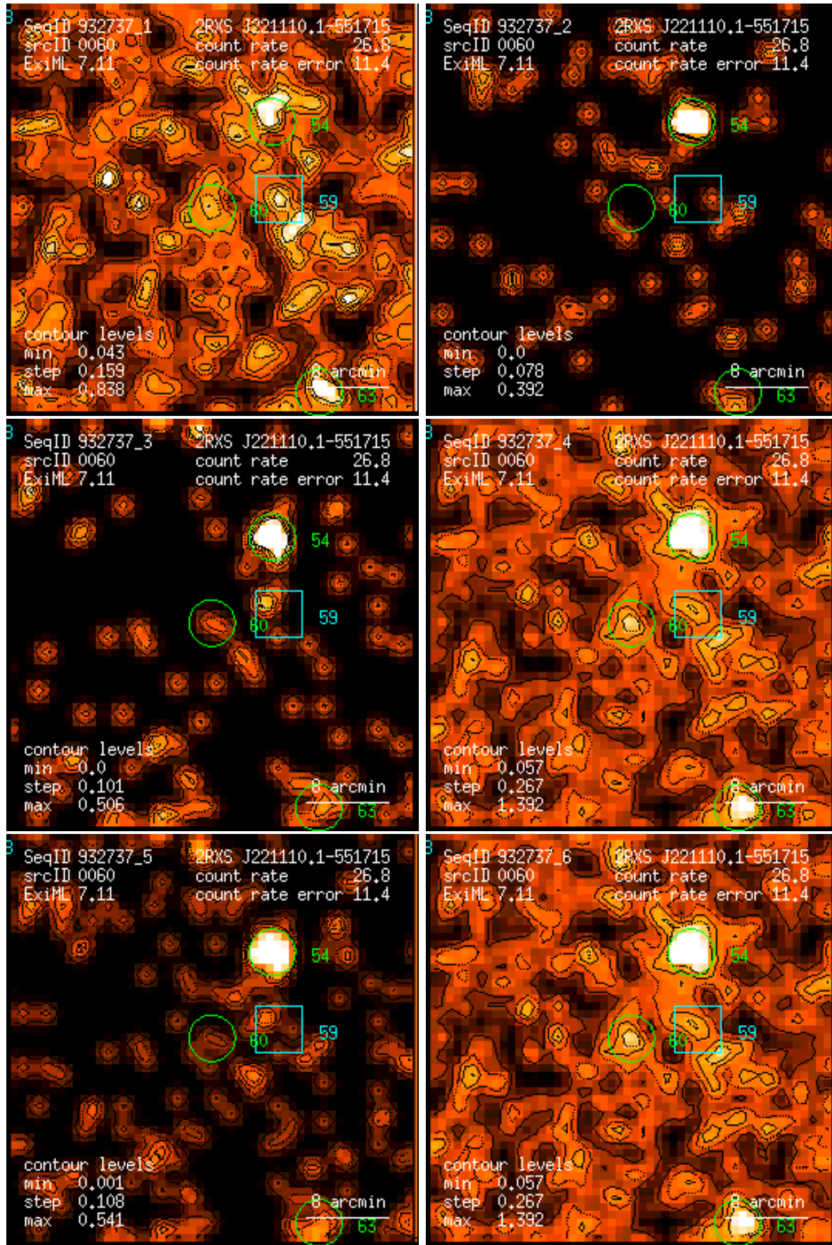
Figure 60: RASS 932737: detection 0060: band rate images, Gaussian filter: (1) PSPC channels 11 – 41, (2) 52 – 90, (3) 91 – 201, (4) 11 – 235, (5) 52 – 201, (6) 11 – 201. Broad band rates in counts/ks. Band rate contour levels in counts/ks/arcmin 2 .
