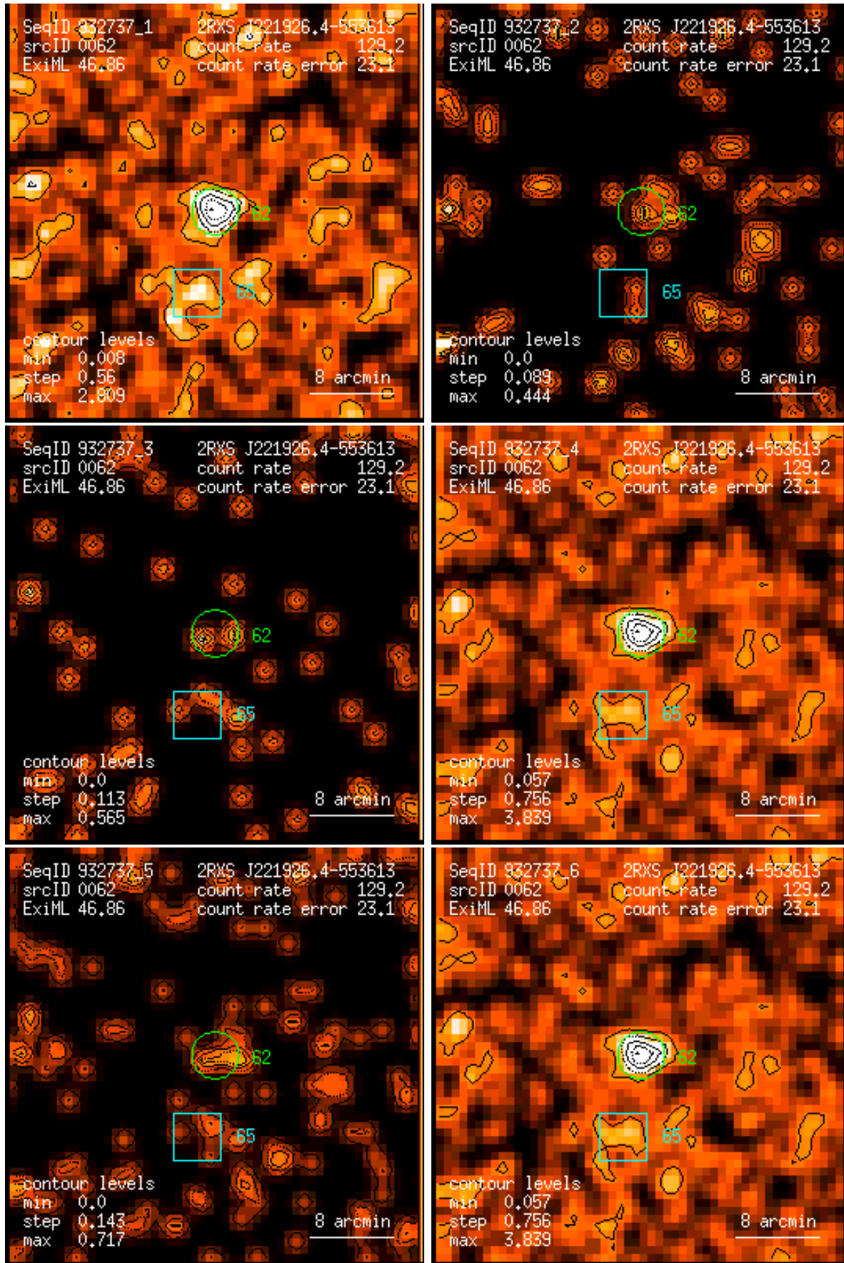
Figure 62: RASS 932737: detection 0062: band rate images, Gaussian filter: (1) PSPC channels 11 – 41, (2) 52 – 90, (3) 91 – 201, (4) 11 – 235, (5) 52 – 201, (6) 11 – 201. Broad band rates in counts/ks. Band rate contour levels in counts/ks/arcmin 2 .
