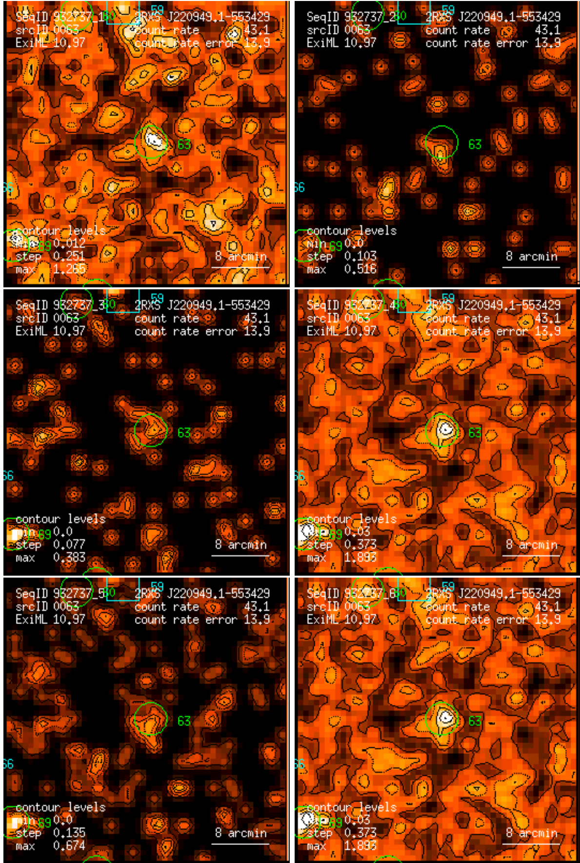
Figure 63: RASS 932737: detection 0063: band rate images, Gaussian filter: (1) PSPC channels 11 – 41, (2) 52 – 90, (3) 91 – 201, (4) 11 – 235, (5) 52 – 201, (6) 11 – 201. Broad band rates in counts/ks. Band rate contour levels in counts/ks/arcmin 2 .
