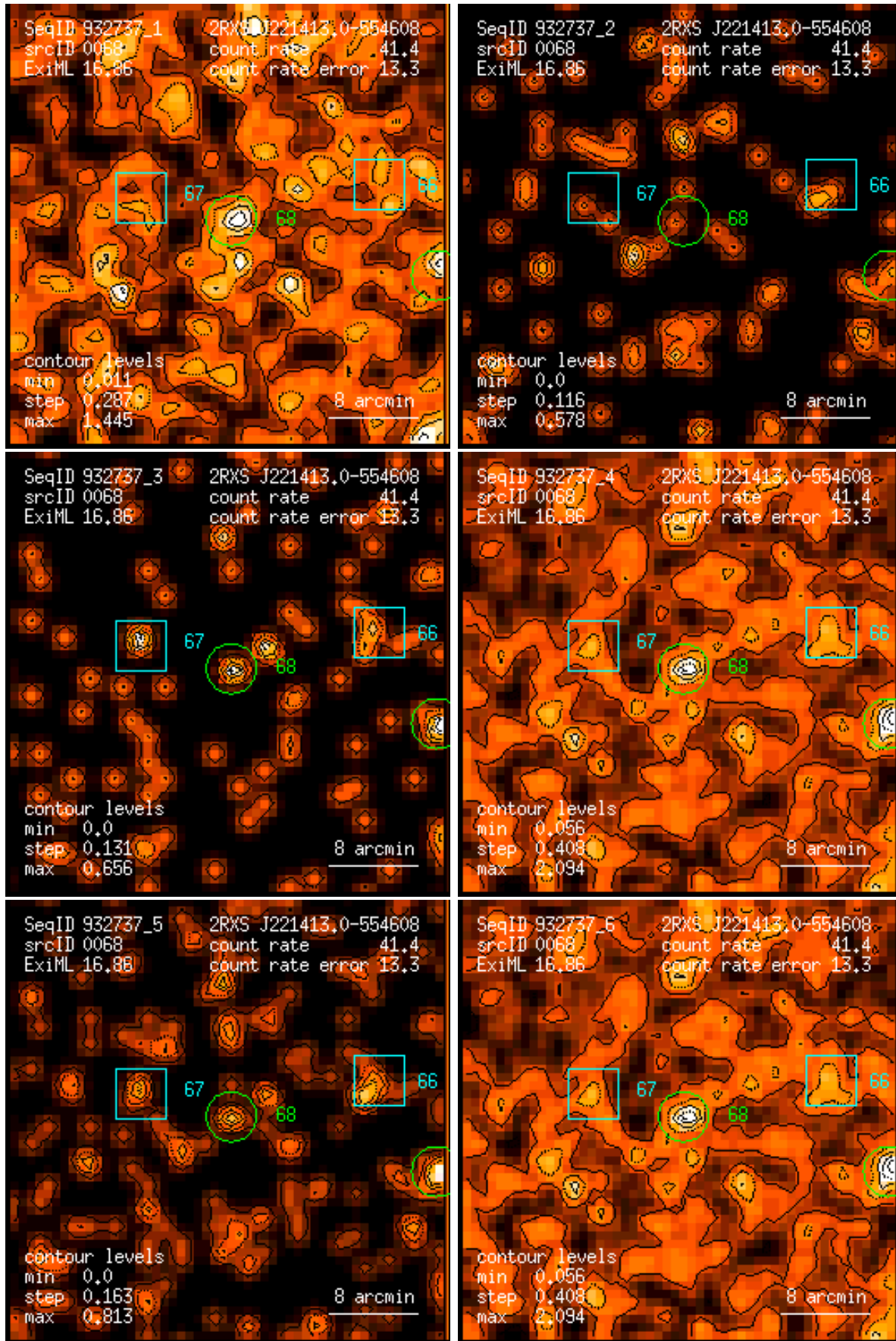
Figure 68: RASS 932737: detection 0068: band rate images, Gaussian filter: (1) PSPC channels 11 – 41, (2) 52 – 90, (3) 91 – 201, (4) 11 – 235, (5) 52 – 201, (6) 11 – 201. Broad band rates in counts/ks. Band rate contour levels in counts/ks/arcmin 2 .
