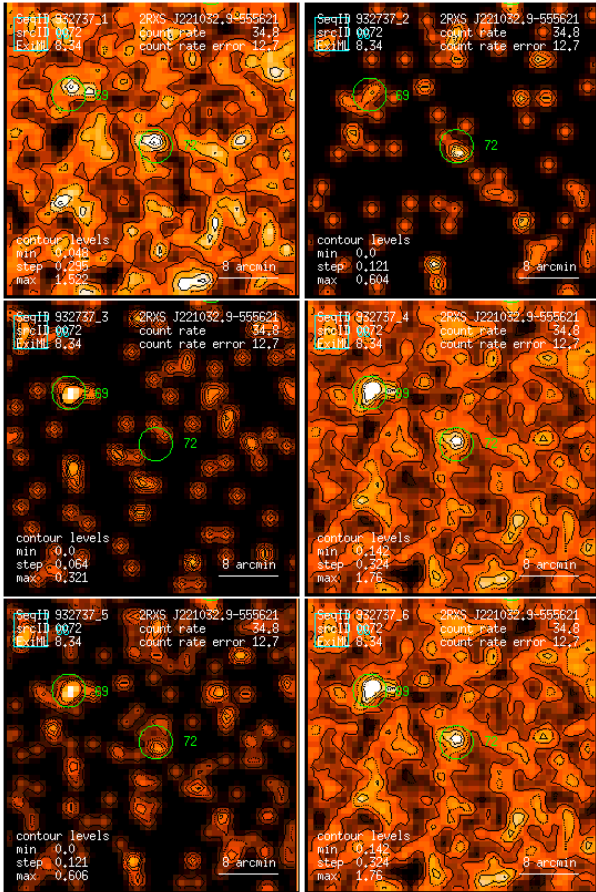
Figure 72: RASS 932737: detection 0072: band rate images, Gaussian filter: (1) PSPC channels 11 – 41, (2) 52 – 90, (3) 91 – 201, (4) 11 – 235, (5) 52 – 201, (6) 11 – 201. Broad band rates in counts/ks. Band rate contour levels in counts/ks/arcmin 2 .
