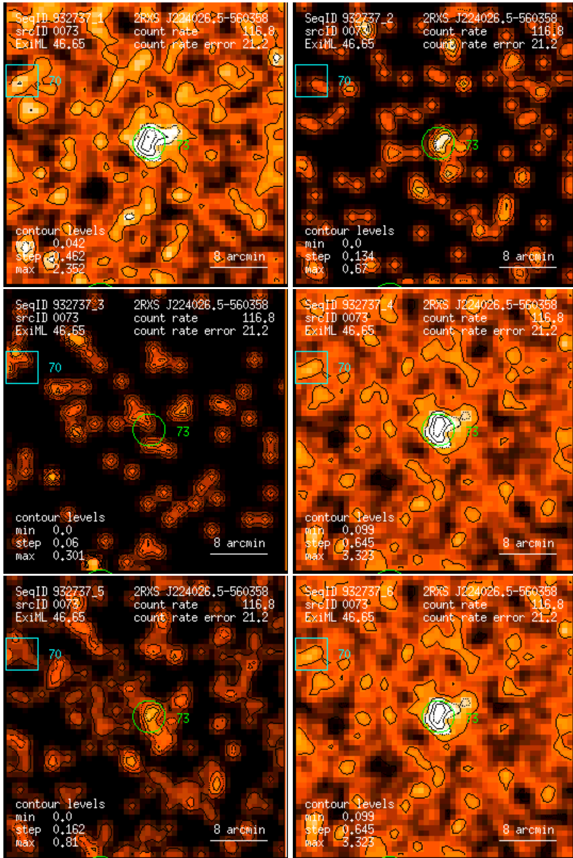
Figure 73: RASS 932737: detection 0073: band rate images, Gaussian filter: (1) PSPC channels 11 – 41, (2) 52 – 90, (3) 91 – 201, (4) 11 – 235, (5) 52 – 201, (6) 11 – 201. Broad band rates in counts/ks. Band rate contour levels in counts/ks/arcmin 2 .
