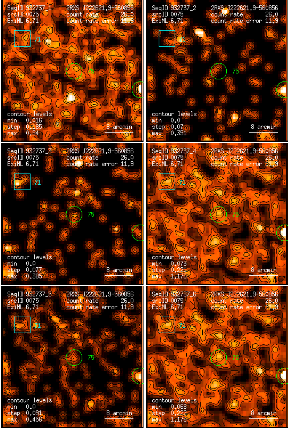
Figure 75: RASS 932737: detection 0075: band rate images, Gaussian filter: (1) PSPC channels 11 – 41, (2) 52 – 90, (3) 91 – 201, (4) 11 – 235, (5) 52 – 201, (6) 11 – 201. Broad band rates in counts/ks. Band rate contour levels in counts/ks/arcmin 2 .
