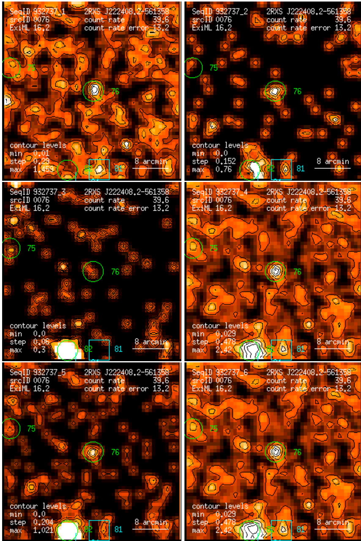
Figure 76: RASS 932737: detection 0076: band rate images, Gaussian filter: (1) PSPC channels 11 – 41, (2) 52 – 90, (3) 91 – 201, (4) 11 – 235, (5) 52 – 201, (6) 11 – 201. Broad band rates in counts/ks. Band rate contour levels in counts/ks/arcmin 2 .
