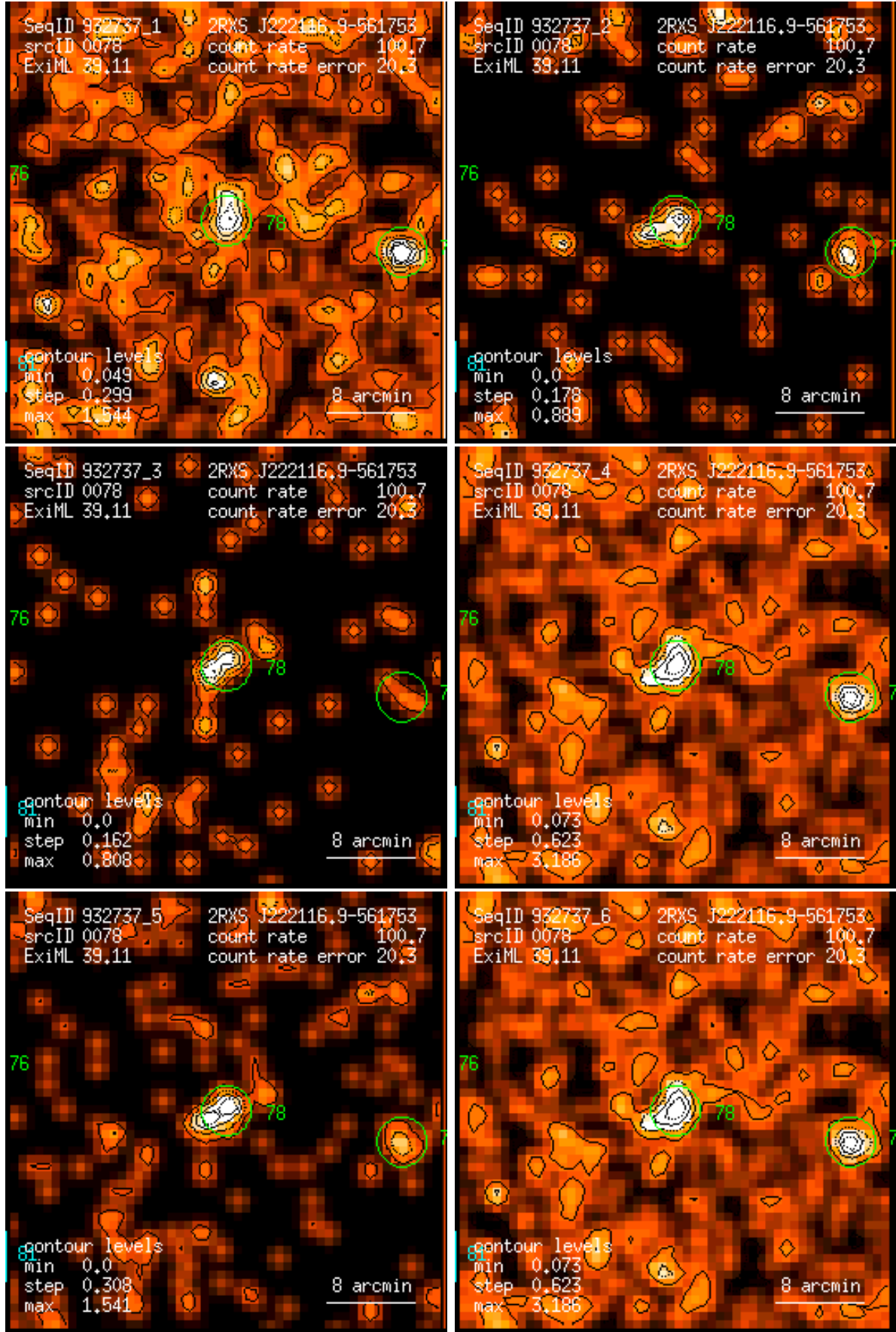
Figure 78: RASS 932737: detection 0078: band rate images, Gaussian filter: (1) PSPC channels 11 – 41, (2) 52 – 90, (3) 91 – 201, (4) 11 – 235, (5) 52 – 201, (6) 11 – 201. Broad band rates in counts/ks. Band rate contour levels in counts/ks/arcmin 2 .
