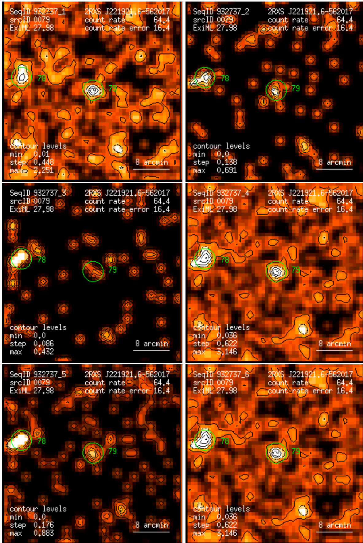
Figure 79: RASS 932737: detection 0079: band rate images, Gaussian filter: (1) PSPC channels 11 – 41, (2) 52 – 90, (3) 91 – 201, (4) 11 – 235, (5) 52 – 201, (6) 11 – 201. Broad band rates in counts/ks. Band rate contour levels in counts/ks/arcmin 2 .
