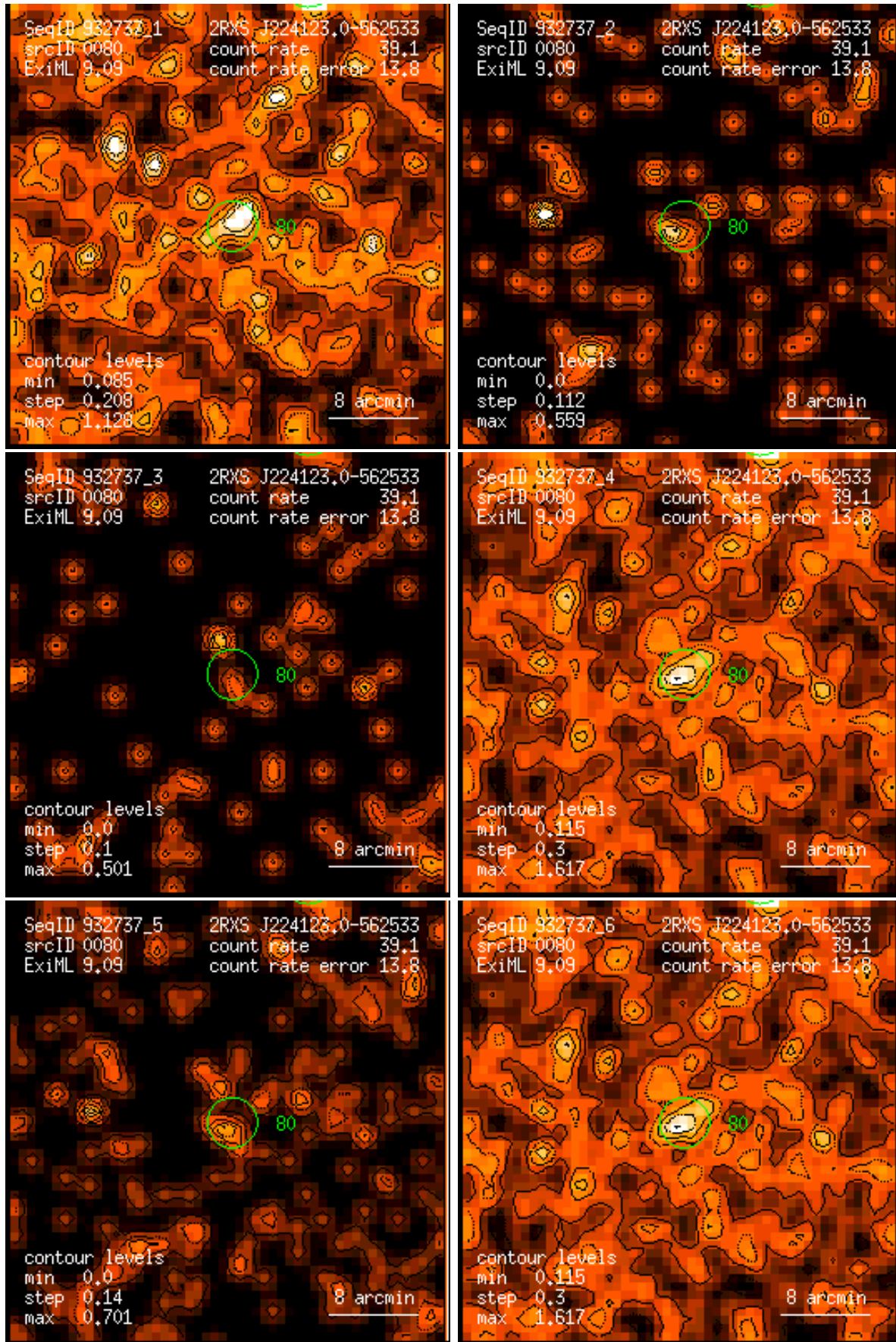
Figure 80: RASS 932737: detection 0080: band rate images, Gaussian filter: (1) PSPC channels 11 – 41, (2) 52 – 90, (3) 91 – 201, (4) 11 – 235, (5) 52 – 201, (6) 11 – 201. Broad band rates in counts/ks. Band rate contour levels in counts/ks/arcmin 2 .
