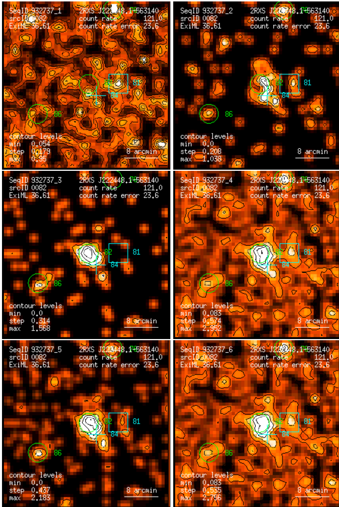
Figure 82: RASS 932737: detection 0082: band rate images, Gaussian filter: (1) PSPC channels 11 – 41, (2) 52 – 90, (3) 91 – 201, (4) 11 – 235, (5) 52 – 201, (6) 11 – 201. Broad band rates in counts/ks. Band rate contour levels in counts/ks/arcmin 2 .
