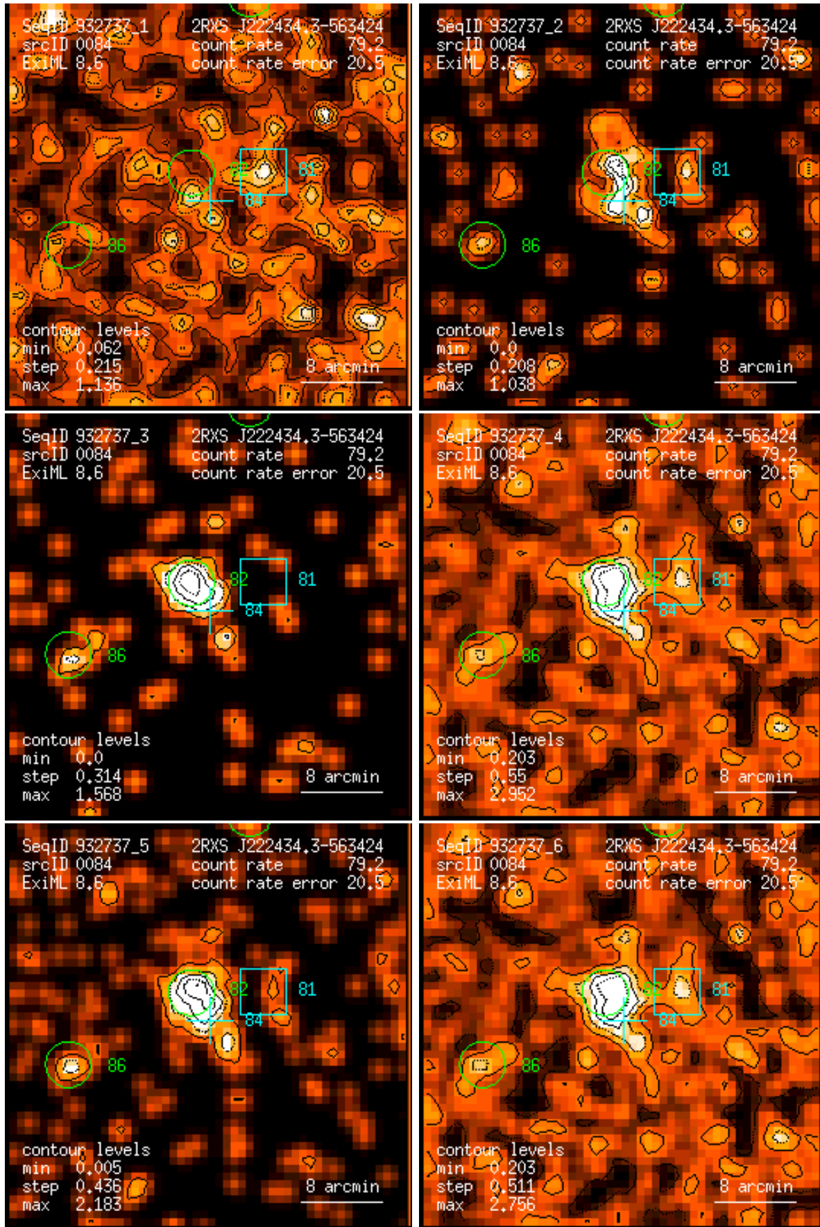
Figure 84: RASS 932737: detection 0084: band rate images, Gaussian filter: (1) PSPC channels 11 – 41, (2) 52 – 90, (3) 91 – 201, (4) 11 – 235, (5) 52 – 201, (6) 11 – 201. Broad band rates in counts/ks. Band rate contour levels in counts/ks/arcmin 2 .
