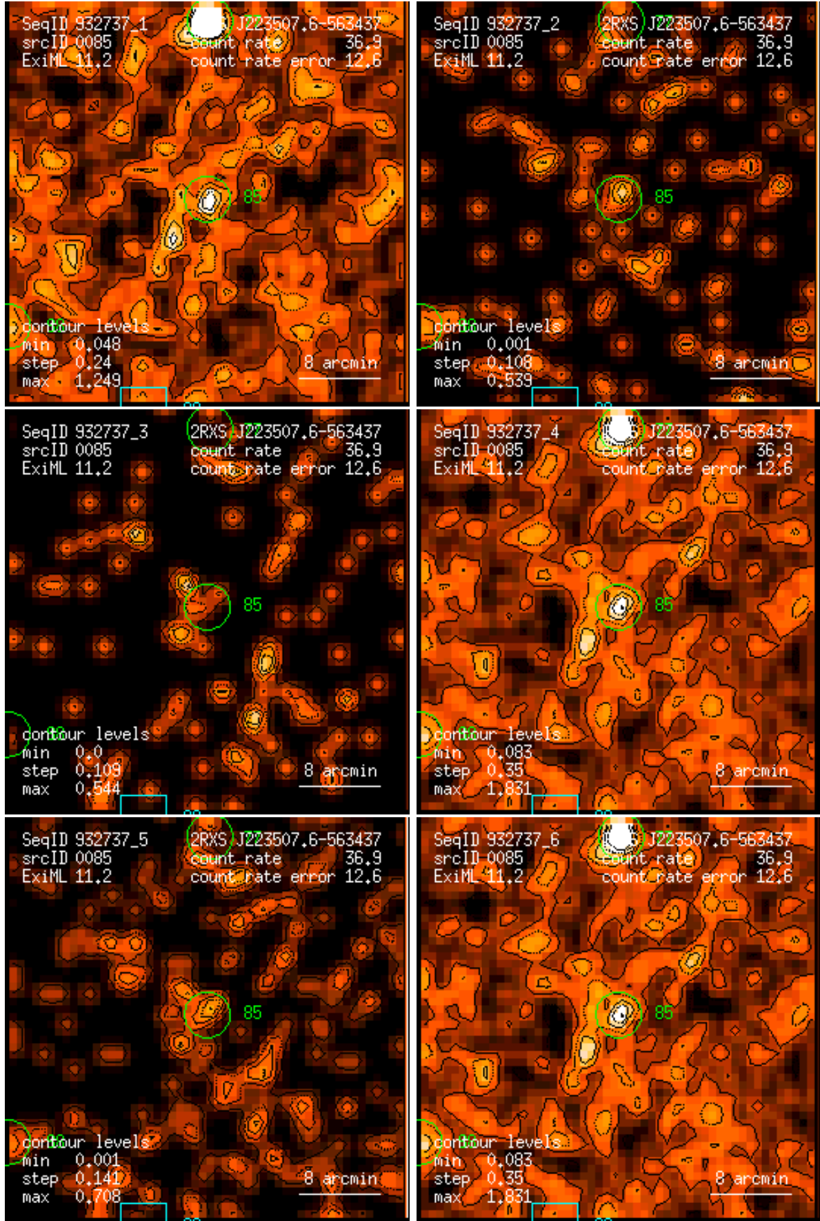
Figure 85: RASS 932737: detection 0085: band rate images, Gaussian filter: (1) PSPC channels 11 – 41, (2) 52 – 90, (3) 91 – 201, (4) 11 – 235, (5) 52 – 201, (6) 11 – 201. Broad band rates in counts/ks. Band rate contour levels in counts/ks/arcmin 2 .
