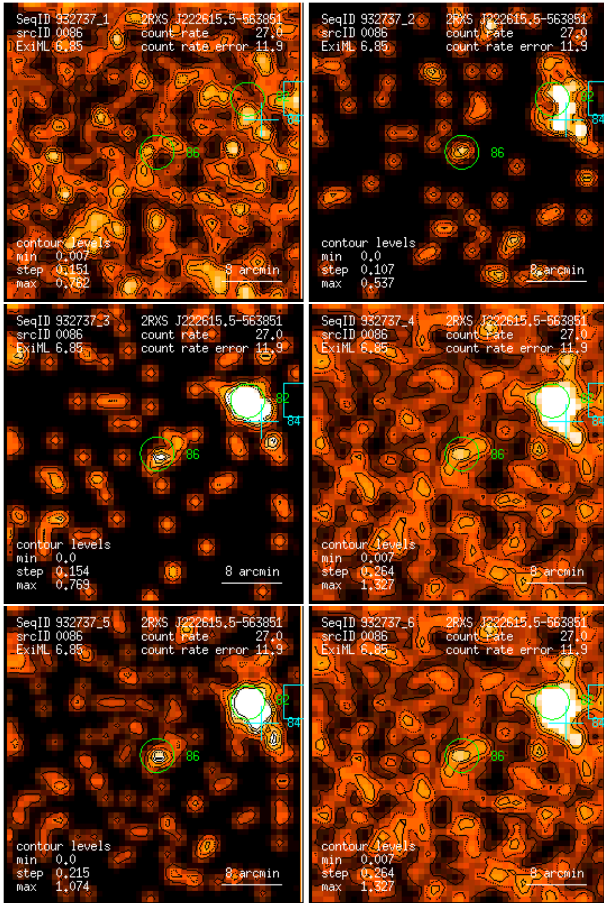
Figure 86: RASS 932737: detection 0086: band rate images, Gaussian filter: (1) PSPC channels 11 – 41, (2) 52 – 90, (3) 91 – 201, (4) 11 – 235, (5) 52 – 201, (6) 11 – 201. Broad band rates in counts/ks. Band rate contour levels in counts/ks/arcmin 2 .
