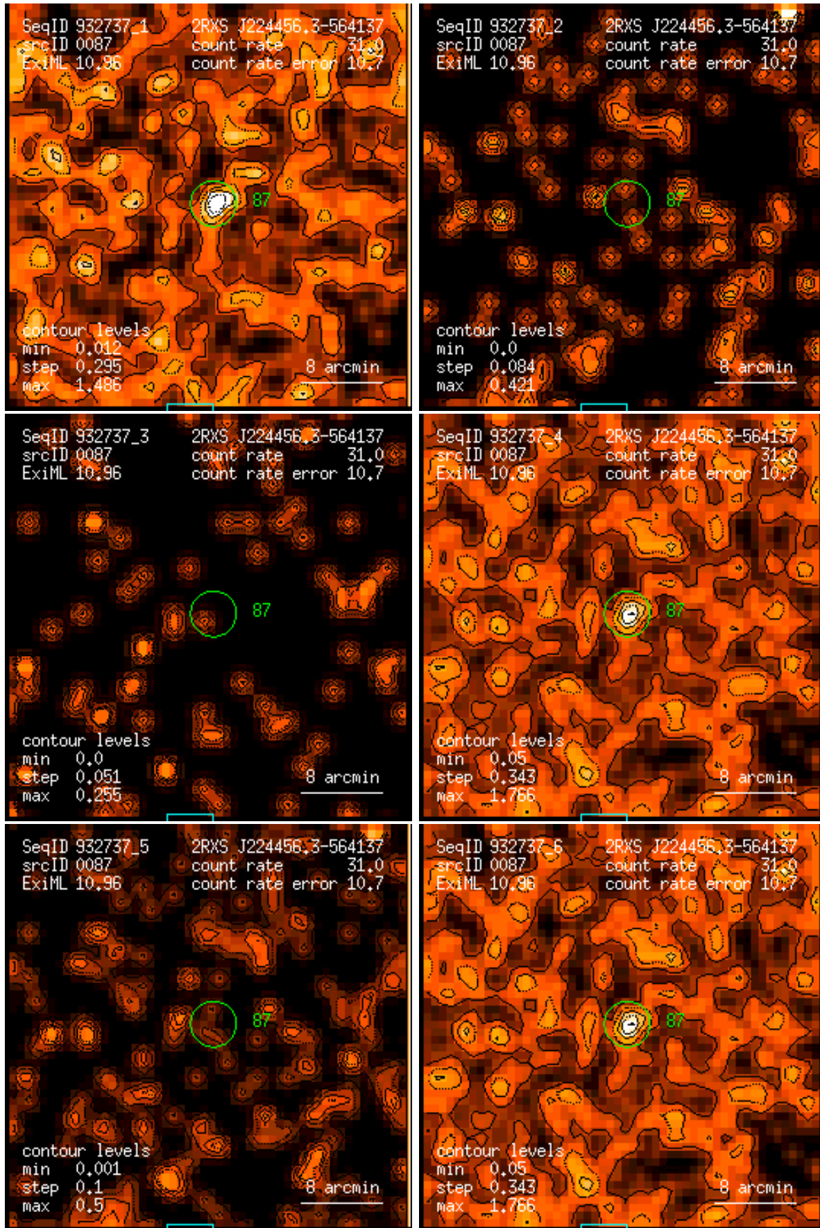
Figure 87: RASS 932737: detection 0087: band rate images, Gaussian filter: (1) PSPC channels 11 – 41, (2) 52 – 90, (3) 91 – 201, (4) 11 – 235, (5) 52 – 201, (6) 11 – 201. Broad band rates in counts/ks. Band rate contour levels in counts/ks/arcmin 2 .
