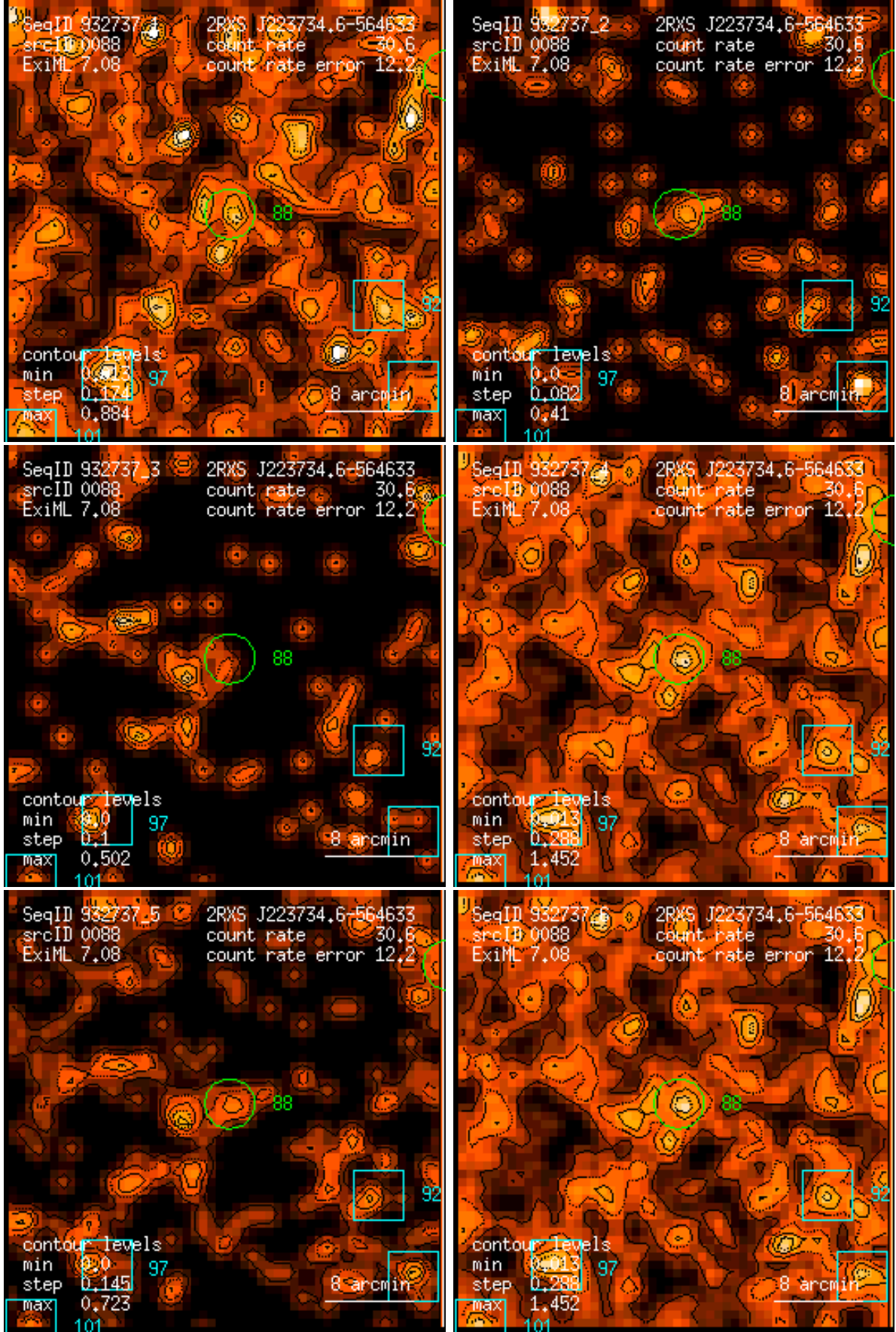
Figure 88: RASS 932737: detection 0088: band rate images, Gaussian filter: (1) PSPC channels 11 – 41, (2) 52 – 90, (3) 91 – 201, (4) 11 – 235, (5) 52 – 201, (6) 11 – 201. Broad band rates in counts/ks. Band rate contour levels in counts/ks/arcmin 2 .
