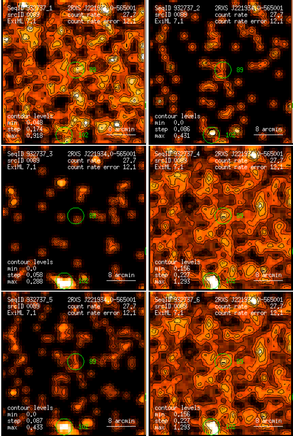
Figure 89: RASS 932737: detection 0089: band rate images, Gaussian filter: (1) PSPC channels 11 – 41, (2) 52 – 90, (3) 91 – 201, (4) 11 – 235, (5) 52 – 201, (6) 11 – 201. Broad band rates in counts/ks. Band rate contour levels in counts/ks/arcmin 2 .
