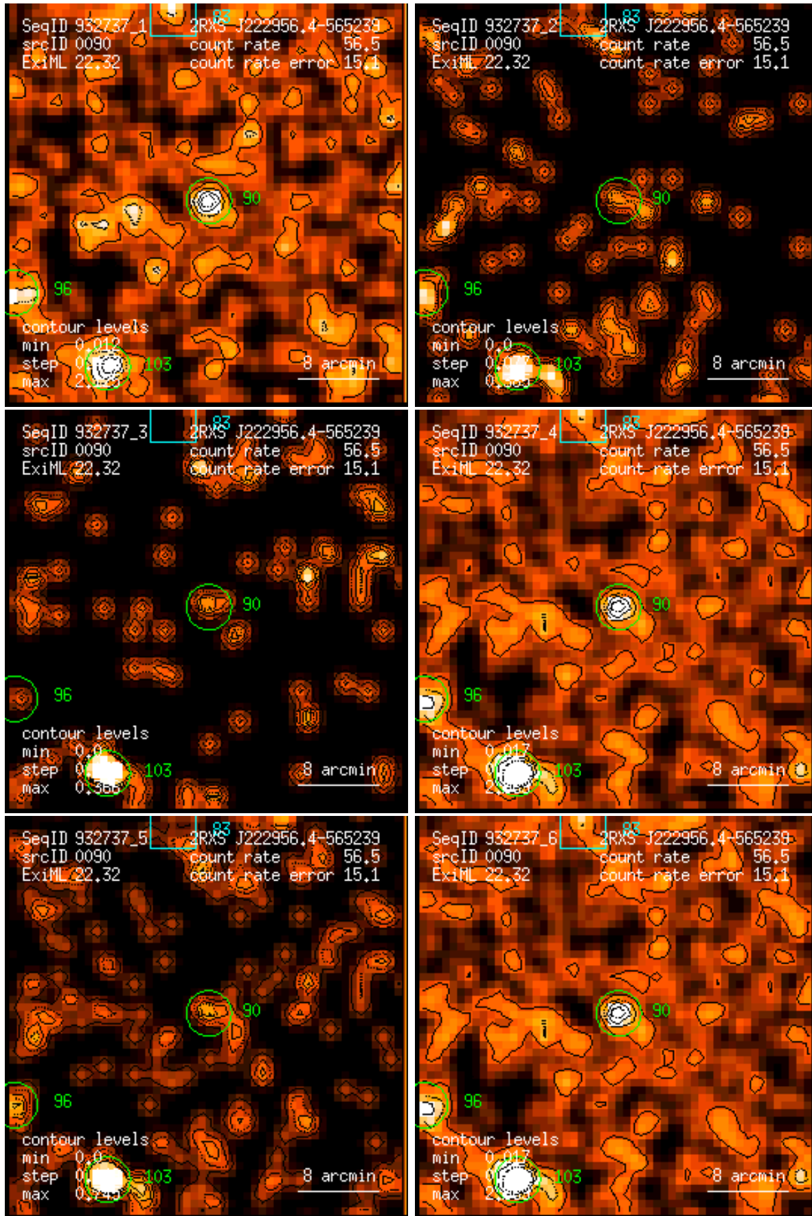
Figure 90: RASS 932737: detection 0090: band rate images, Gaussian filter: (1) PSPC channels 11 – 41, (2) 52 – 90, (3) 91 – 201, (4) 11 – 235, (5) 52 – 201, (6) 11 – 201. Broad band rates in counts/ks. Band rate contour levels in counts/ks/arcmin 2 .
