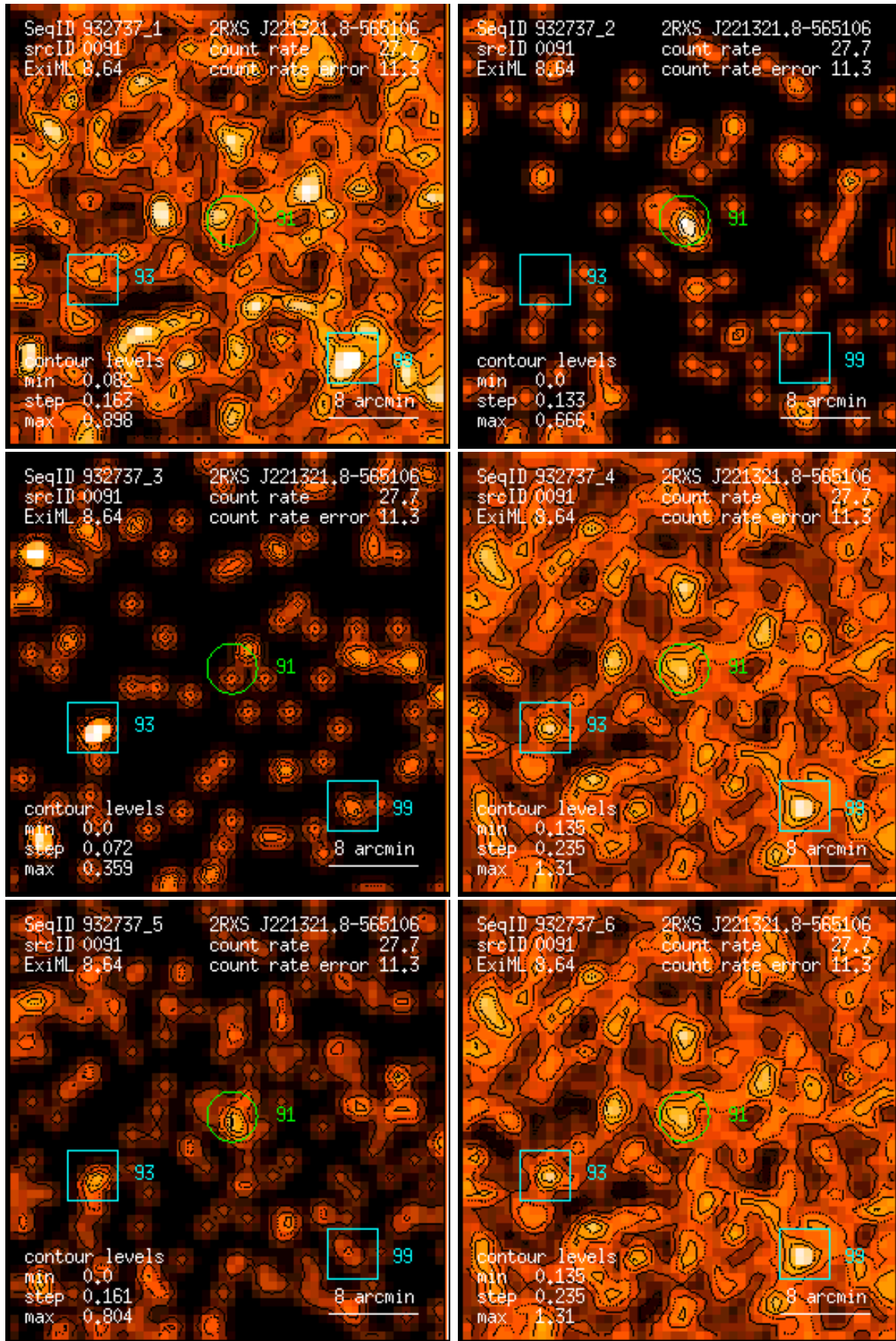
Figure 91: RASS 932737: detection 0091: band rate images, Gaussian filter: (1) PSPC channels 11 – 41, (2) 52 – 90, (3) 91 – 201, (4) 11 – 235, (5) 52 – 201, (6) 11 – 201. Broad band rates in counts/ks. Band rate contour levels in counts/ks/arcmin 2 .
