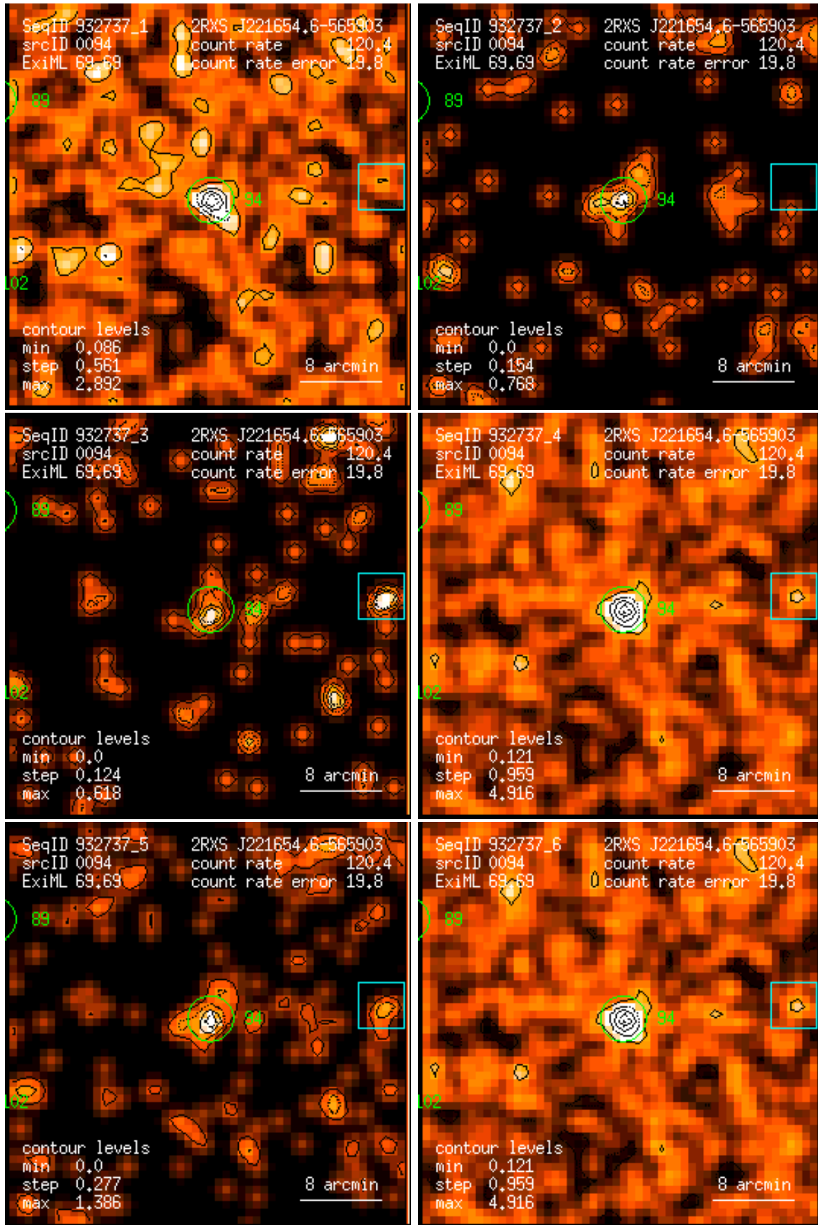
Figure 94: RASS 932737: detection 0094: band rate images, Gaussian filter: (1) PSPC channels 11 – 41, (2) 52 – 90, (3) 91 – 201, (4) 11 – 235, (5) 52 – 201, (6) 11 – 201. Broad band rates in counts/ks. Band rate contour levels in counts/ks/arcmin 2 .
