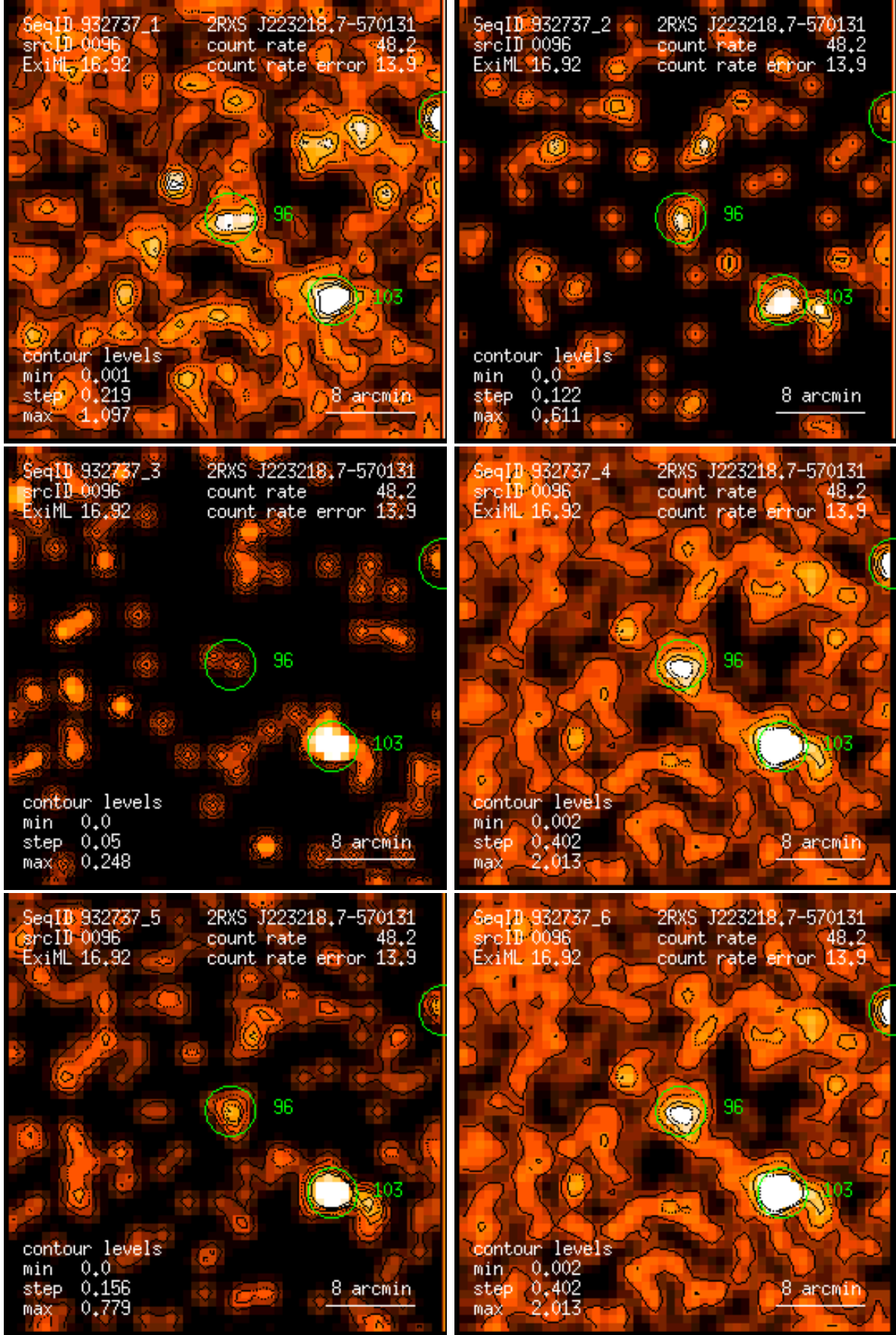
Figure 96: RASS 932737: detection 0096: band rate images, Gaussian filter: (1) PSPC channels 11 – 41, (2) 52 – 90, (3) 91 – 201, (4) 11 – 235, (5) 52 – 201, (6) 11 – 201. Broad band rates in counts/ks. Band rate contour levels in counts/ks/arcmin 2 .
