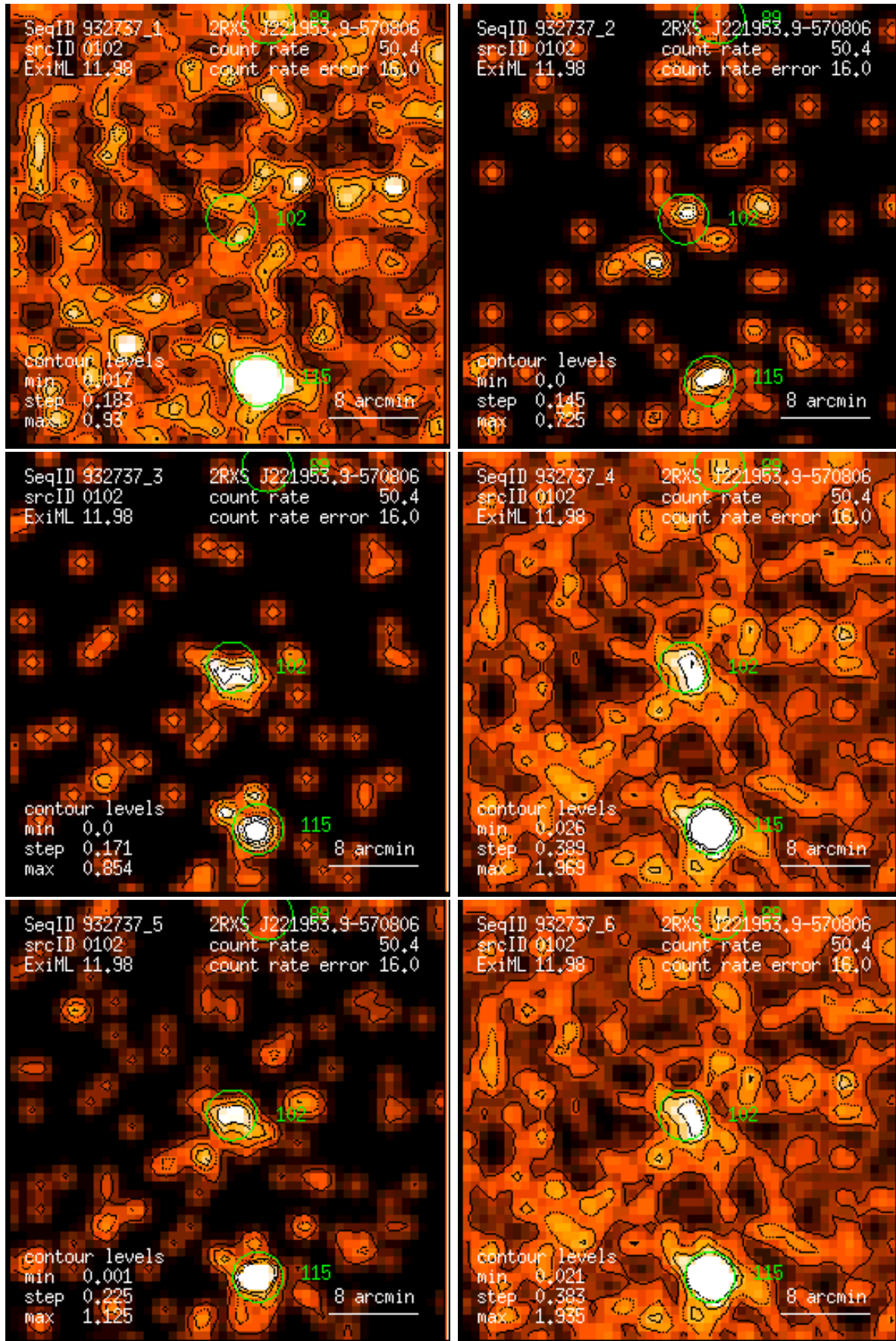
Figure 102: RASS 932737: detection 0102: band rate images, Gaussian filter: (1) PSPC channels 11 – 41, (2) 52 – 90, (3) 91 – 201, (4) 11 – 235, (5) 52 – 201, (6) 11 – 201. Broad band rates in counts/ks. Band rate contour levels in counts/ks/arcmin 2 .
