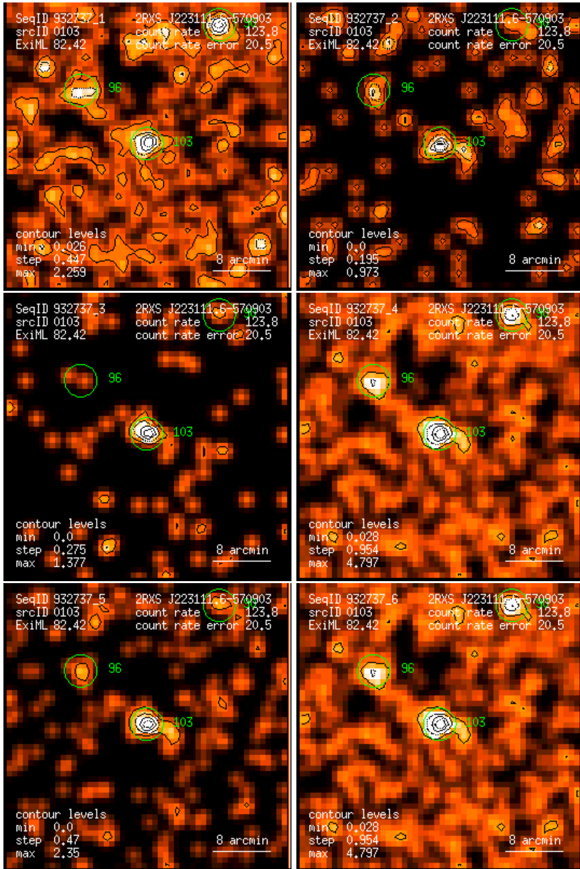
Figure 103: RASS 932737: detection 0103: band rate images, Gaussian filter: (1) PSPC channels 11 – 41, (2) 52 – 90, (3) 91 – 201, (4) 11 – 235, (5) 52 – 201, (6) 11 – 201. Broad band rates in counts/ks. Band rate contour levels in counts/ks/arcmin 2 .
