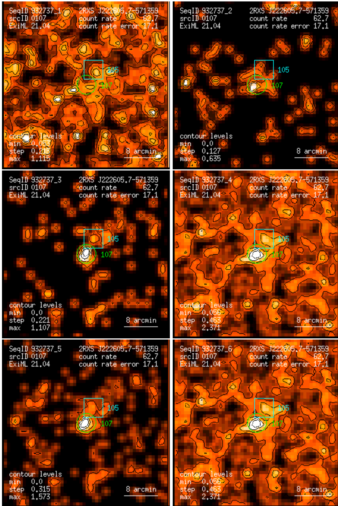
Figure 107: RASS 932737: detection 0107: band rate images, Gaussian filter: (1) PSPC channels 11 – 41, (2) 52 – 90, (3) 91 – 201, (4) 11 – 235, (5) 52 – 201, (6) 11 – 201. Broad band rates in counts/ks. Band rate contour levels in counts/ks/arcmin 2 .
