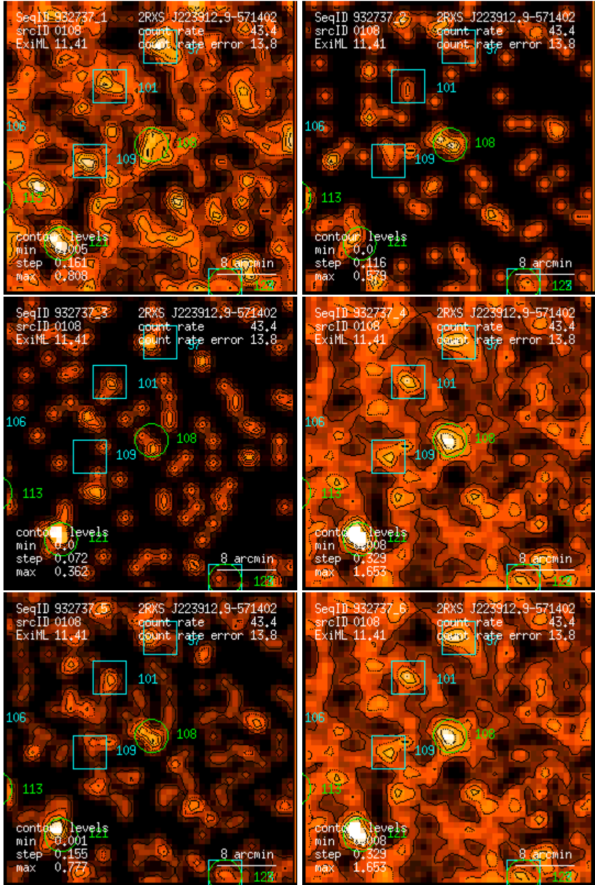
Figure 108: RASS 932737: detection 0108: band rate images, Gaussian filter: (1) PSPC channels 11 – 41, (2) 52 – 90, (3) 91 – 201, (4) 11 – 235, (5) 52 – 201, (6) 11 – 201. Broad band rates in counts/ks. Band rate contour levels in counts/ks/arcmin 2 .
