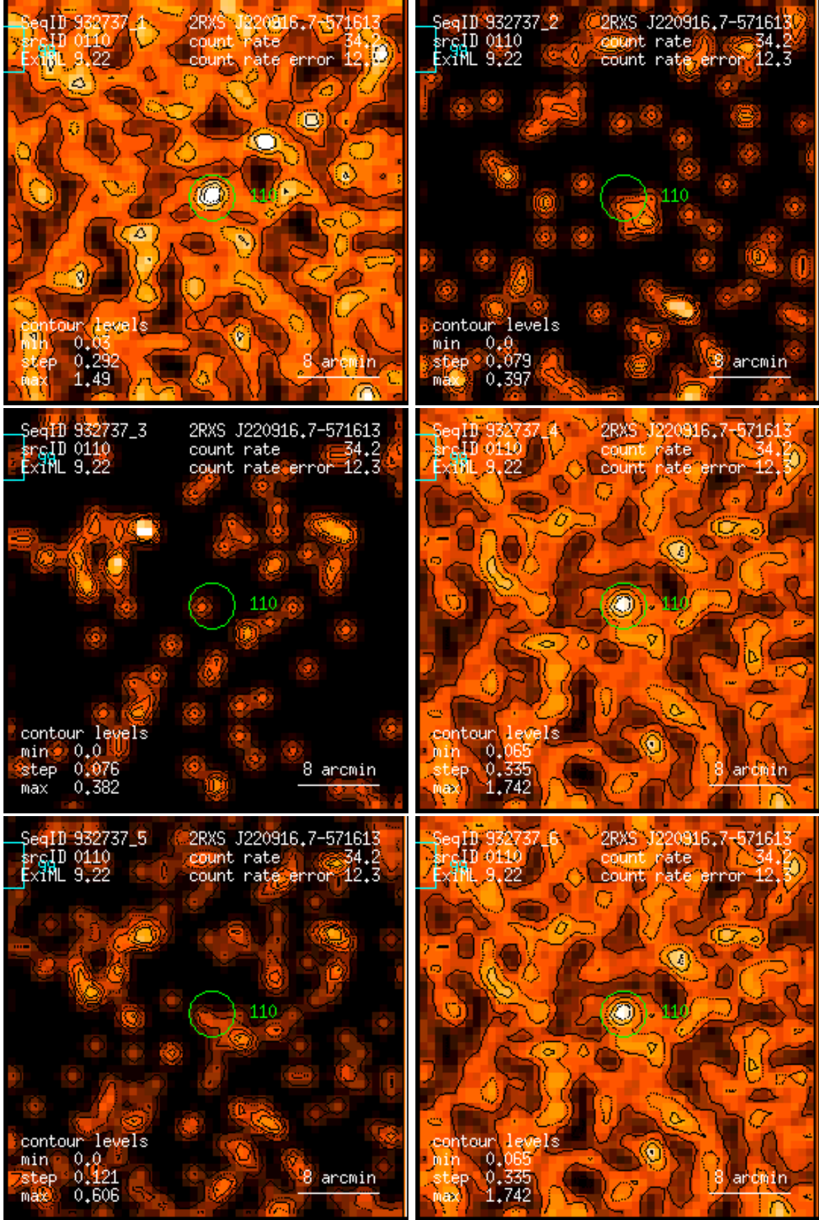
Figure 110: RASS 932737: detection 0110: band rate images, Gaussian filter: (1) PSPC channels 11 – 41, (2) 52 – 90, (3) 91 – 201, (4) 11 – 235, (5) 52 – 201, (6) 11 – 201. Broad band rates in counts/ks. Band rate contour levels in counts/ks/arcmin 2 .
