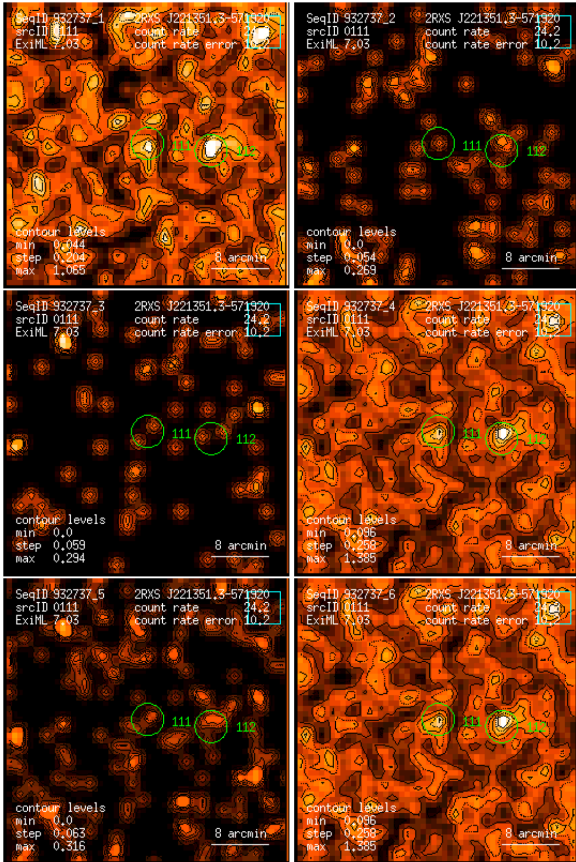
Figure 111: RASS 932737: detection 0111: band rate images, Gaussian filter: (1) PSPC channels 11 – 41, (2) 52 – 90, (3) 91 – 201, (4) 11 – 235, (5) 52 – 201, (6) 11 – 201. Broad band rates in counts/ks. Band rate contour levels in counts/ks/arcmin 2 .
