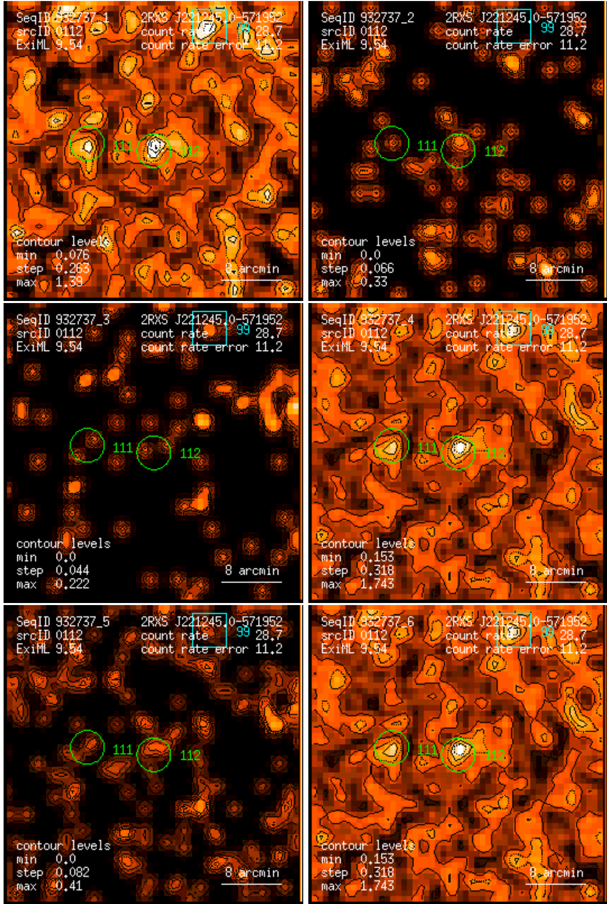
Figure 112: RASS 932737: detection 0112: band rate images, Gaussian filter: (1) PSPC channels 11 – 41, (2) 52 – 90, (3) 91 – 201, (4) 11 – 235, (5) 52 – 201, (6) 11 – 201. Broad band rates in counts/ks. Band rate contour levels in counts/ks/arcmin 2 .
