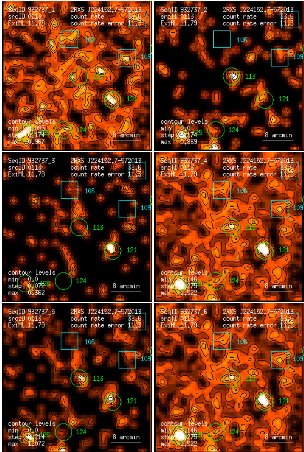
Figure 113: RASS 932737: detection 0113: band rate images, Gaussian filter: (1) PSPC channels 11 – 41, (2) 52 – 90, (3) 91 – 201, (4) 11 – 235, (5) 52 – 201, (6) 11 – 201. Broad band rates in counts/ks. Band rate contour levels in counts/ks/arcmin 2 .
