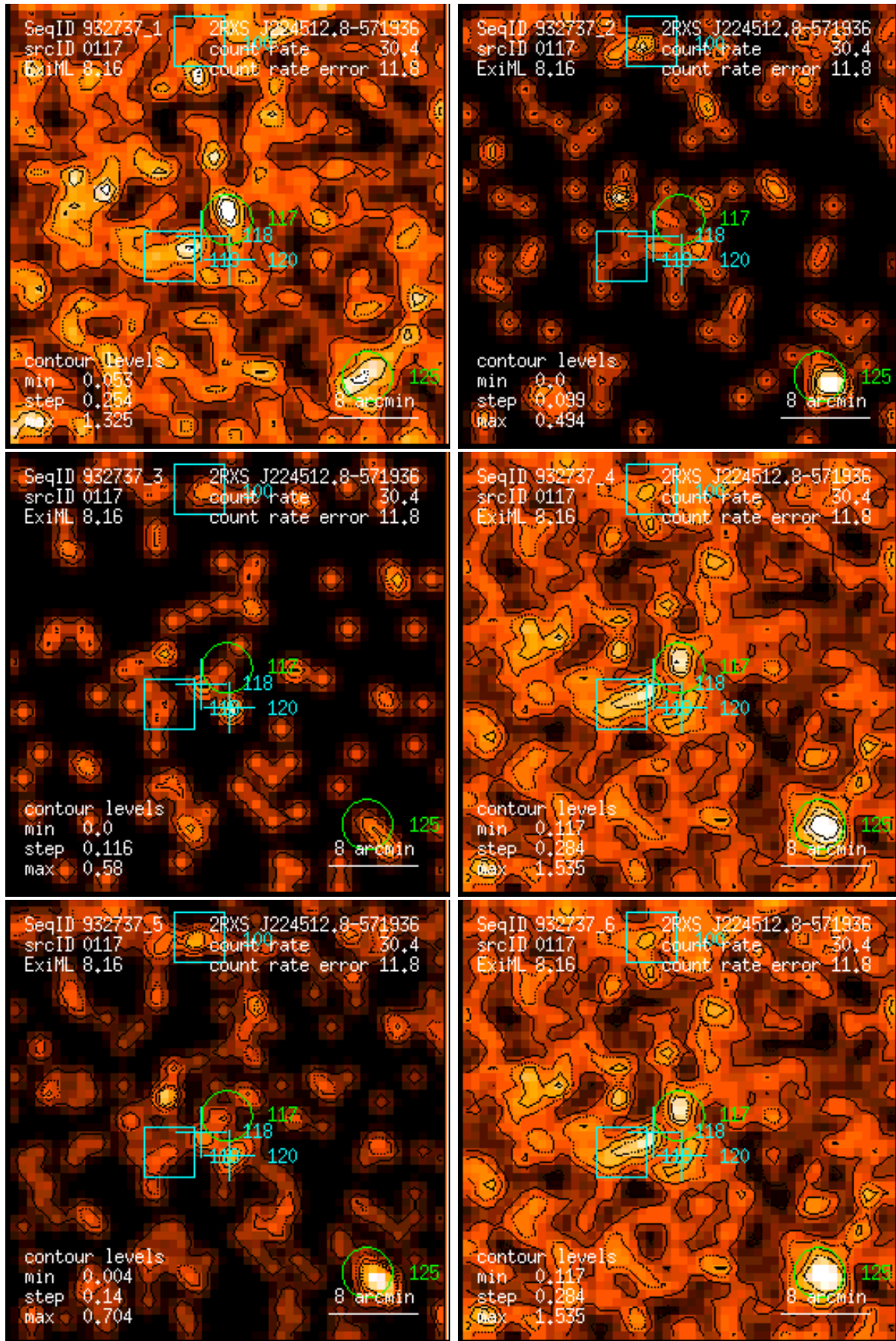
Figure 117: RASS 932737: detection 0117: band rate images, Gaussian filter: (1) PSPC channels 11 – 41, (2) 52 – 90, (3) 91 – 201, (4) 11 – 235, (5) 52 – 201, (6) 11 – 201. Broad band rates in counts/ks. Band rate contour levels in counts/ks/arcmin 2 .
