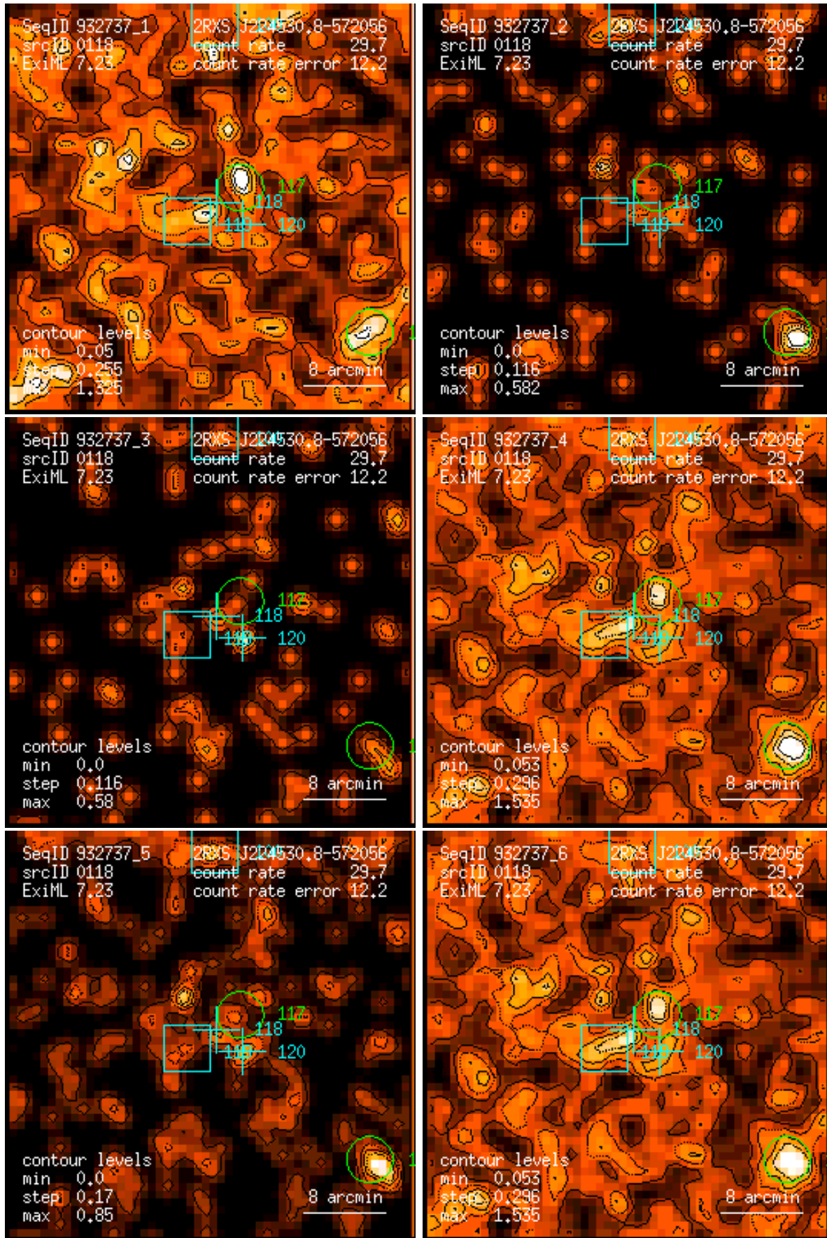
Figure 118: RASS 932737: detection 0118: band rate images, Gaussian filter: (1) PSPC channels 11 – 41, (2) 52 – 90, (3) 91 – 201, (4) 11 – 235, (5) 52 – 201, (6) 11 – 201. Broad band rates in counts/ks. Band rate contour levels in counts/ks/arcmin 2 .
