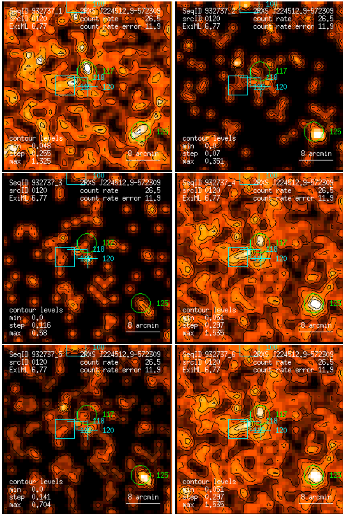
Figure 120: RASS 932737: detection 0120: band rate images, Gaussian filter: (1) PSPC channels 11 – 41, (2) 52 – 90, (3) 91 – 201, (4) 11 – 235, (5) 52 – 201, (6) 11 – 201. Broad band rates in counts/ks. Band rate contour levels in counts/ks/arcmin 2 .
