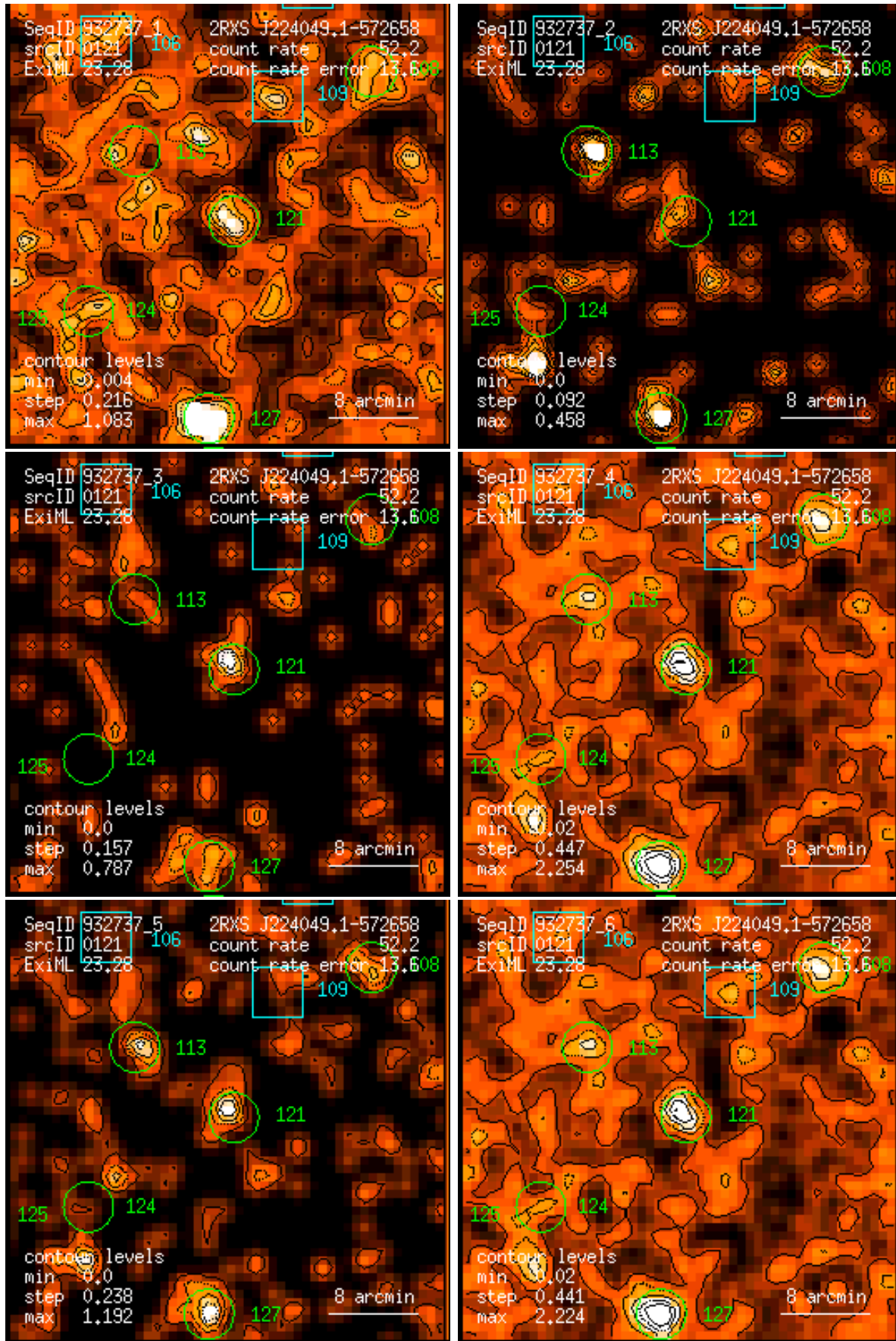
Figure 121: RASS 932737: detection 0121: band rate images, Gaussian filter: (1) PSPC channels 11 – 41, (2) 52 – 90, (3) 91 – 201, (4) 11 – 235, (5) 52 – 201, (6) 11 – 201. Broad band rates in counts/ks. Band rate contour levels in counts/ks/arcmin 2 .
