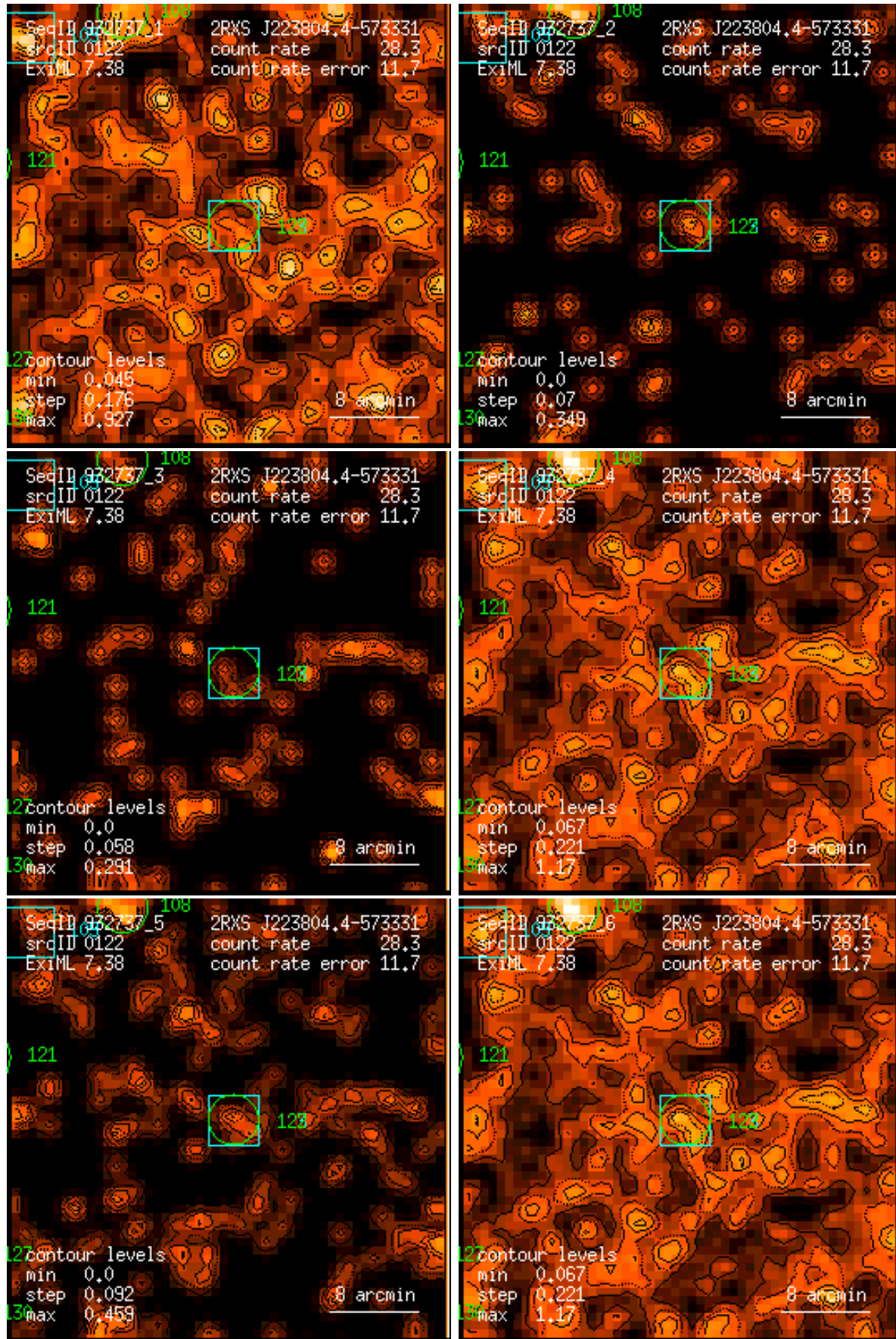
Figure 122: RASS 932737: detection 0122: band rate images, Gaussian filter: (1) PSPC channels 11 – 41, (2) 52 – 90, (3) 91 – 201, (4) 11 – 235, (5) 52 – 201, (6) 11 – 201. Broad band rates in counts/ks. Band rate contour levels in counts/ks/arcmin 2 .
