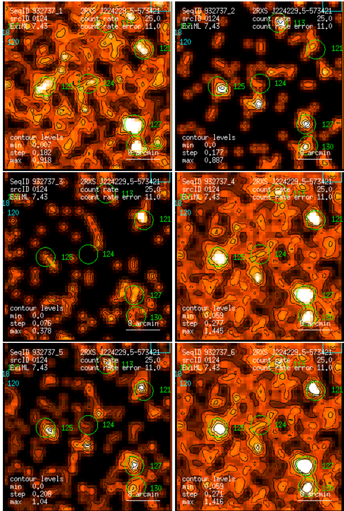
Figure 124: RASS 932737: detection 0124: band rate images, Gaussian filter: (1) PSPC channels 11 – 41, (2) 52 – 90, (3) 91 – 201, (4) 11 – 235, (5) 52 – 201, (6) 11 – 201. Broad band rates in counts/ks. Band rate contour levels in counts/ks/arcmin 2 .
