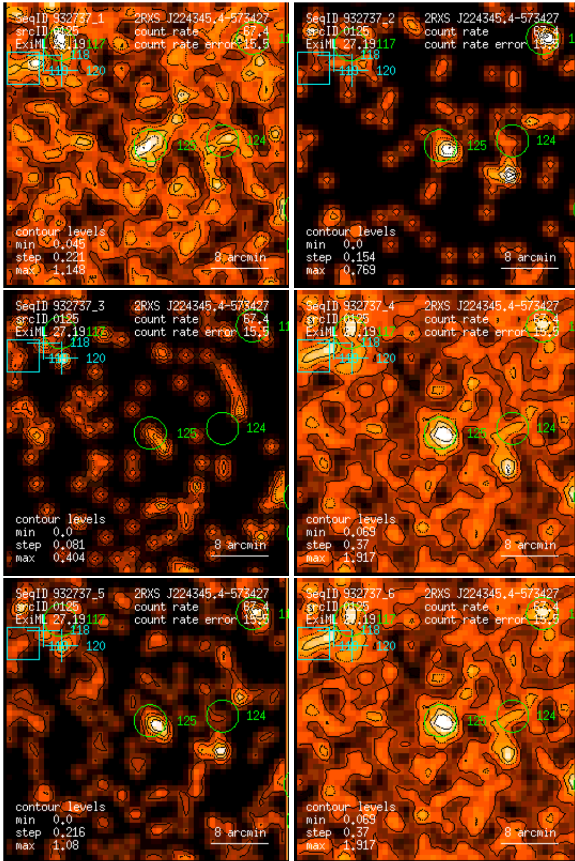
Figure 125: RASS 932737: detection 0125: band rate images, Gaussian filter: (1) PSPC channels 11 – 41, (2) 52 – 90, (3) 91 – 201, (4) 11 – 235, (5) 52 – 201, (6) 11 – 201. Broad band rates in counts/ks. Band rate contour levels in counts/ks/arcmin 2 .
